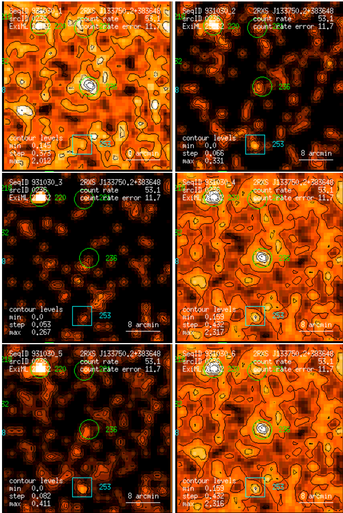
Figure 236: RASS 931030: detection 0236: band rate images, Gaussian filter: (1) PSPC channels 11 – 41, (2) 52 – 90, (3) 91 – 201, (4) 11 – 235, (5) 52 – 201, (6) 11 – 201. Broad band rates in counts/ks. Band rate contour levels in counts/ks/arcmin 2 .
