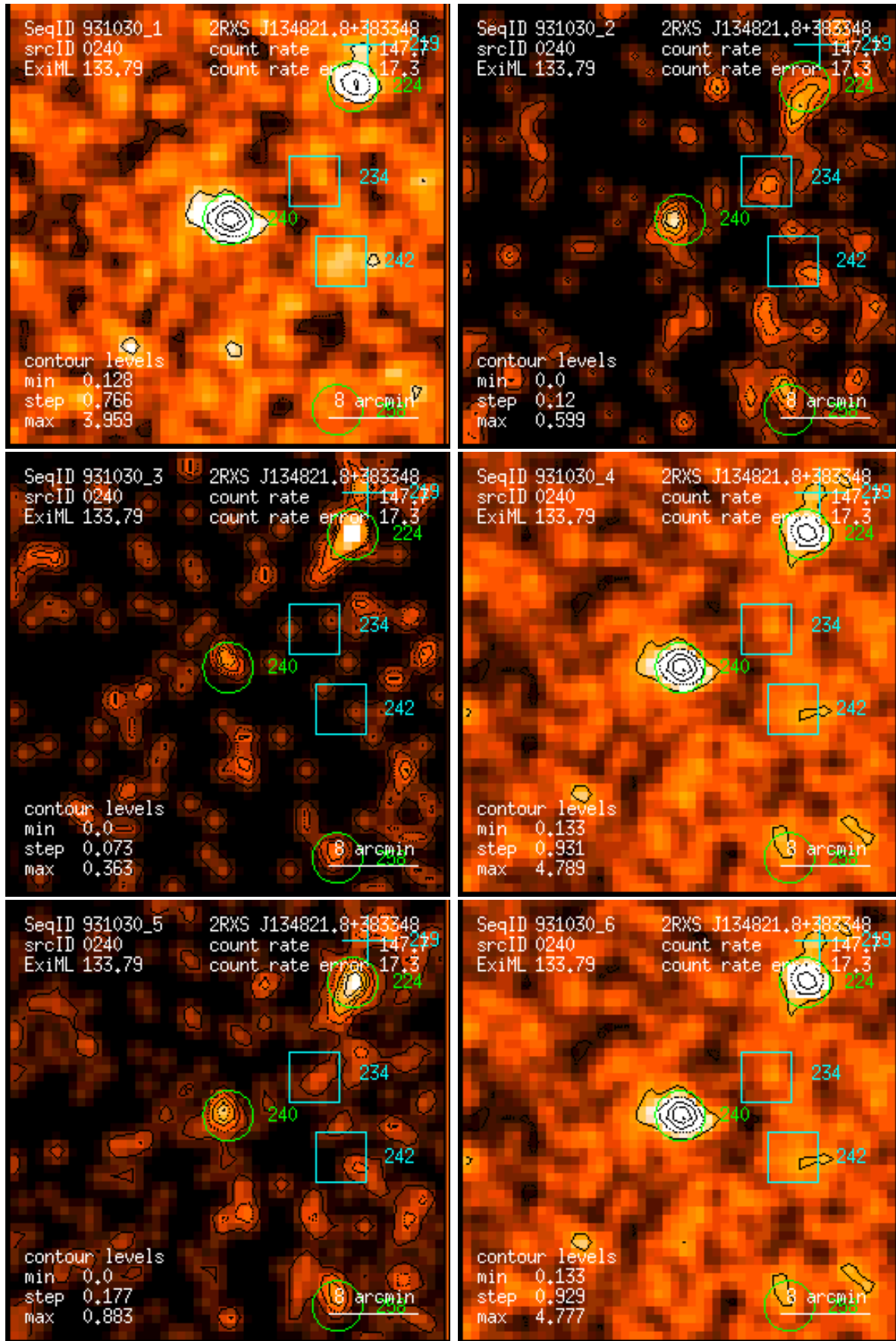
Figure 240: RASS 931030: detection 0240: band rate images, Gaussian filter: (1) PSPC channels 11 – 41, (2) 52 – 90, (3) 91 – 201, (4) 11 – 235, (5) 52 – 201, (6) 11 – 201. Broad band rates in counts/ks. Band rate contour levels in counts/ks/arcmin 2 .
