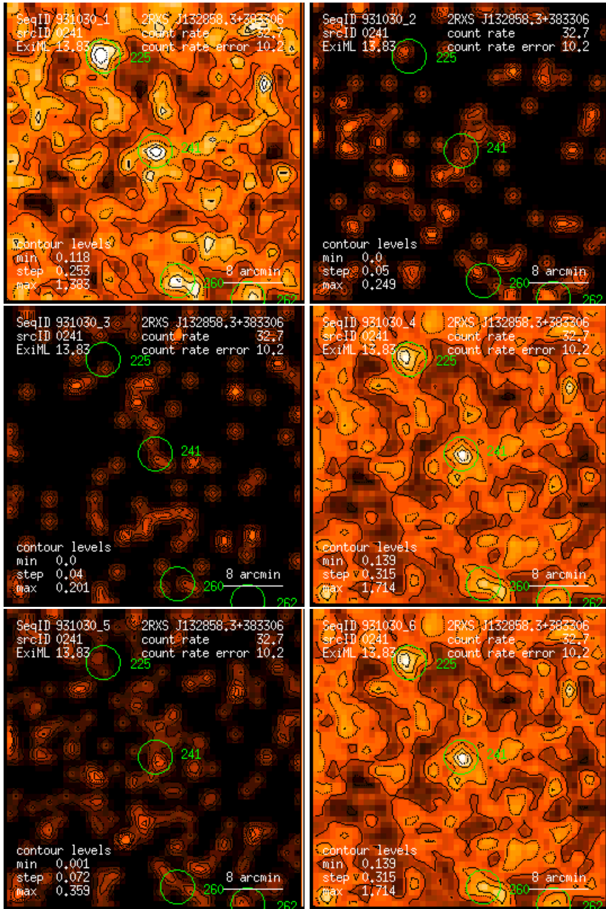
Figure 241: RASS 931030: detection 0241: band rate images, Gaussian filter: (1) PSPC channels 11 – 41, (2) 52 – 90, (3) 91 – 201, (4) 11 – 235, (5) 52 – 201, (6) 11 – 201. Broad band rates in counts/ks. Band rate contour levels in counts/ks/arcmin 2 .
