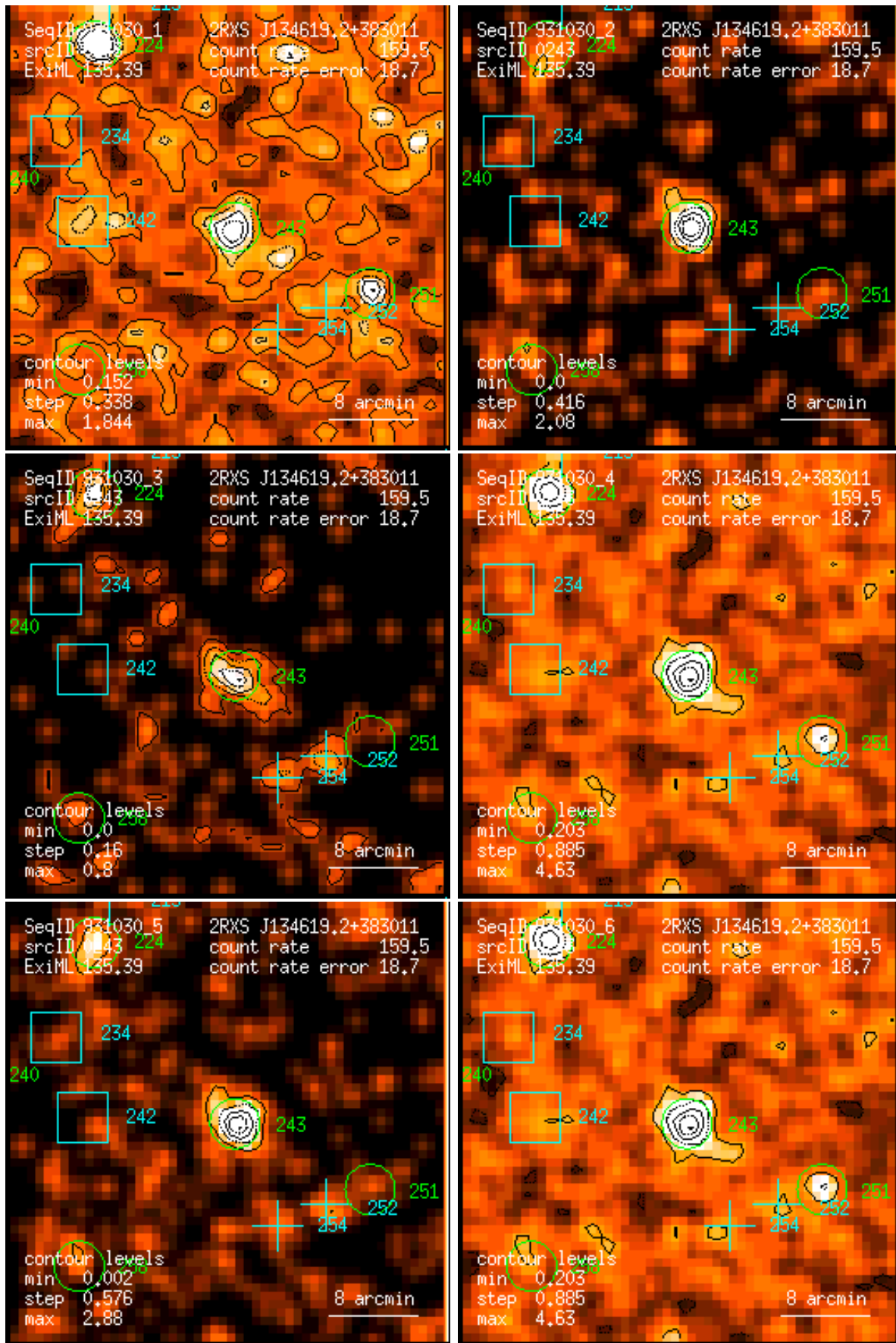
Figure 243: RASS 931030: detection 0243: band rate images, Gaussian filter: (1) PSPC channels 11 – 41, (2) 52 – 90, (3) 91 – 201, (4) 11 – 235, (5) 52 – 201, (6) 11 – 201. Broad band rates in counts/ks. Band rate contour levels in counts/ks/arcmin 2 .
