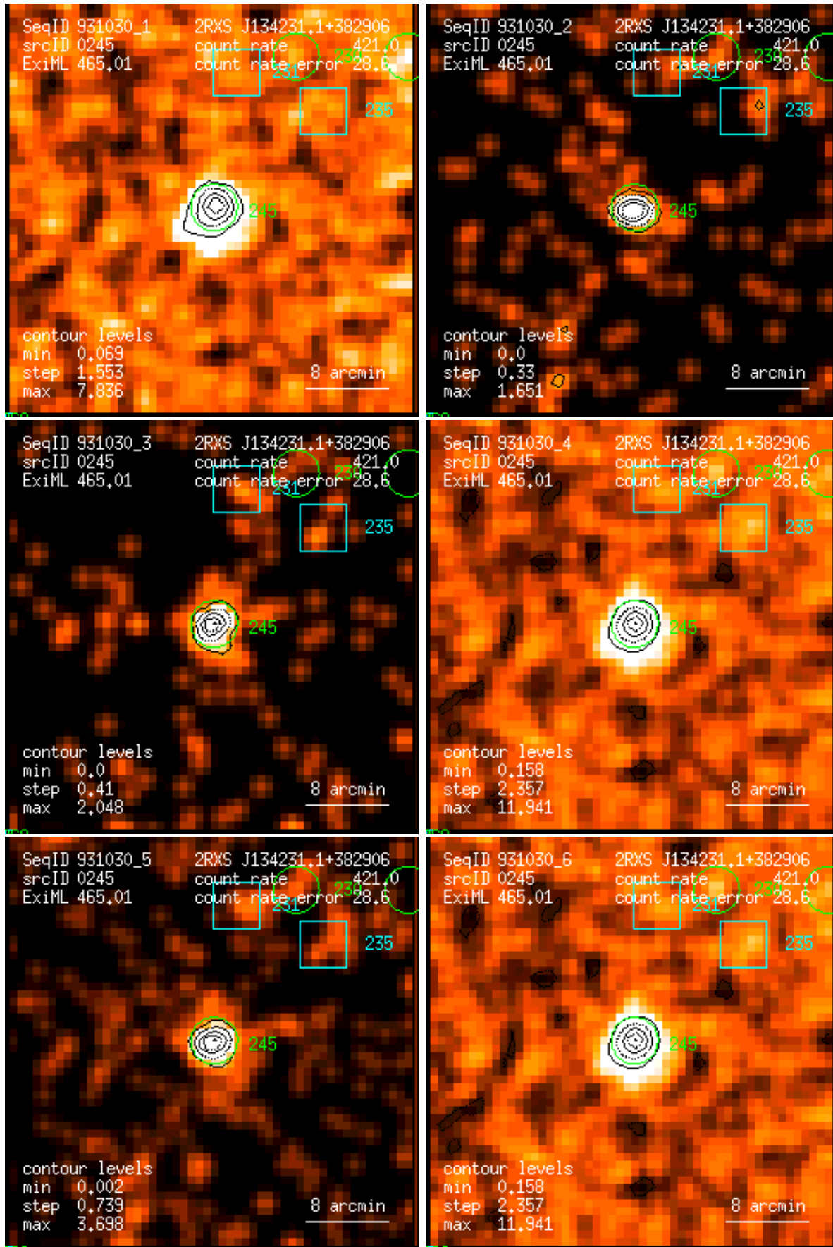
Figure 245: RASS 931030: detection 0245: band rate images, Gaussian filter: (1) PSPC channels 11 – 41, (2) 52 – 90, (3) 91 – 201, (4) 11 – 235, (5) 52 – 201, (6) 11 – 201. Broad band rates in counts/ks. Band rate contour levels in counts/ks/arcmin 2 .
