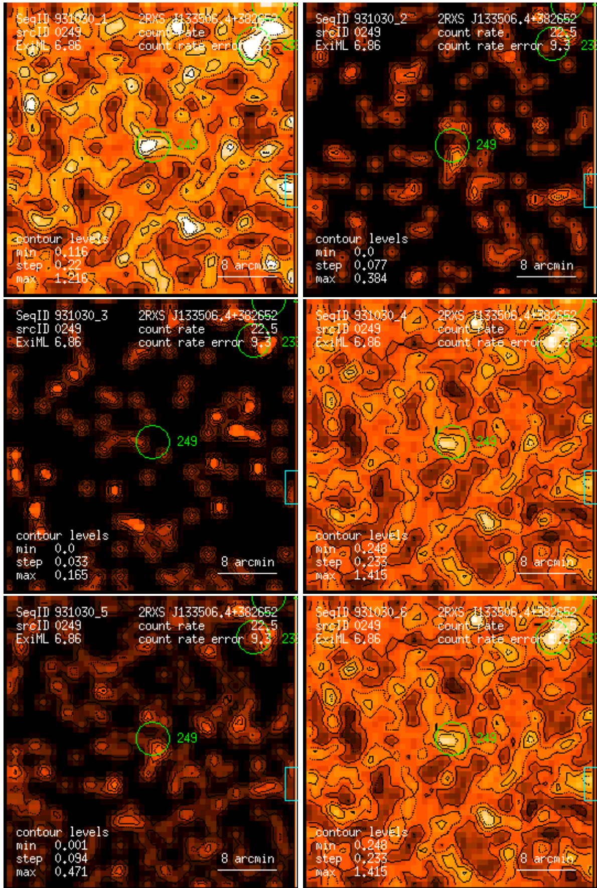
Figure 249: RASS 931030: detection 0249: band rate images, Gaussian filter: (1) PSPC channels 11 – 41, (2) 52 – 90, (3) 91 – 201, (4) 11 – 235, (5) 52 – 201, (6) 11 – 201. Broad band rates in counts/ks. Band rate contour levels in counts/ks/arcmin 2 .
