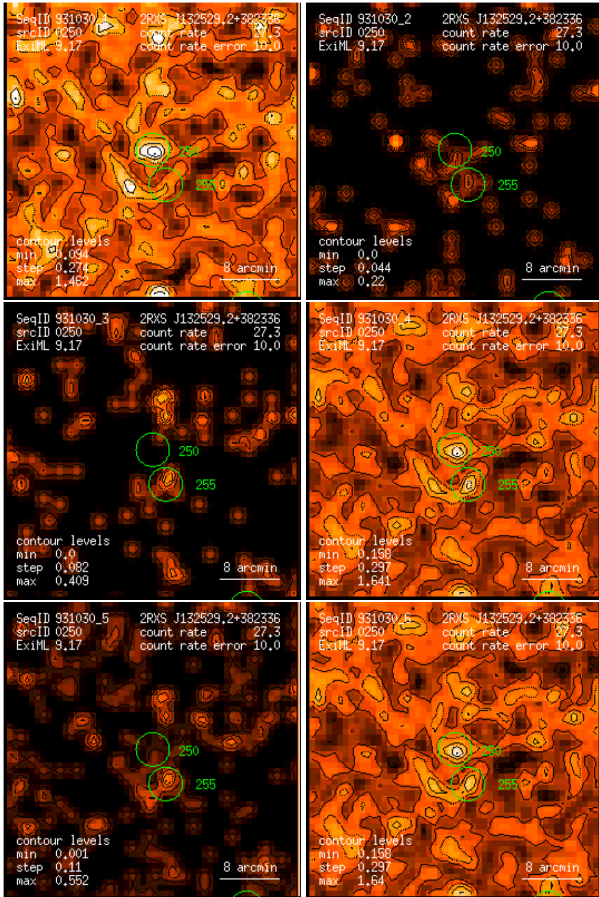
Figure 250: RASS 931030: detection 0250: band rate images, Gaussian filter: (1) PSPC channels 11 – 41, (2) 52 – 90, (3) 91 – 201, (4) 11 – 235, (5) 52 – 201, (6) 11 – 201. Broad band rates in counts/ks. Band rate contour levels in counts/ks/arcmin 2 .
