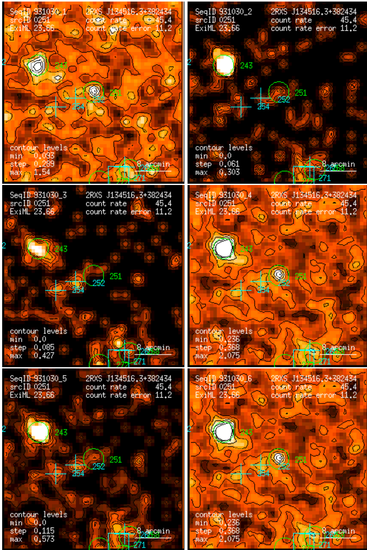
Figure 251: RASS 931030: detection 0251: band rate images, Gaussian filter: (1) PSPC channels 11 – 41, (2) 52 – 90, (3) 91 – 201, (4) 11 – 235, (5) 52 – 201, (6) 11 – 201. Broad band rates in counts/ks. Band rate contour levels in counts/ks/arcmin 2 .
