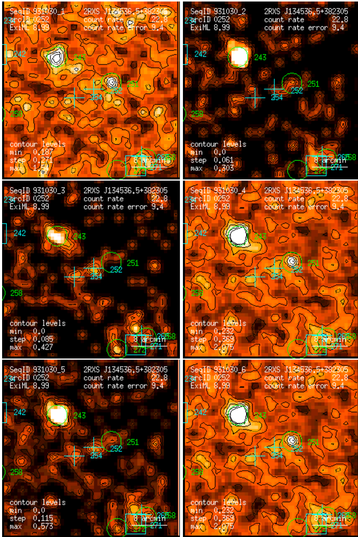
Figure 252: RASS 931030: detection 0252: band rate images, Gaussian filter: (1) PSPC channels 11 – 41, (2) 52 – 90, (3) 91 – 201, (4) 11 – 235, (5) 52 – 201, (6) 11 – 201. Broad band rates in counts/ks. Band rate contour levels in counts/ks/arcmin 2 .
