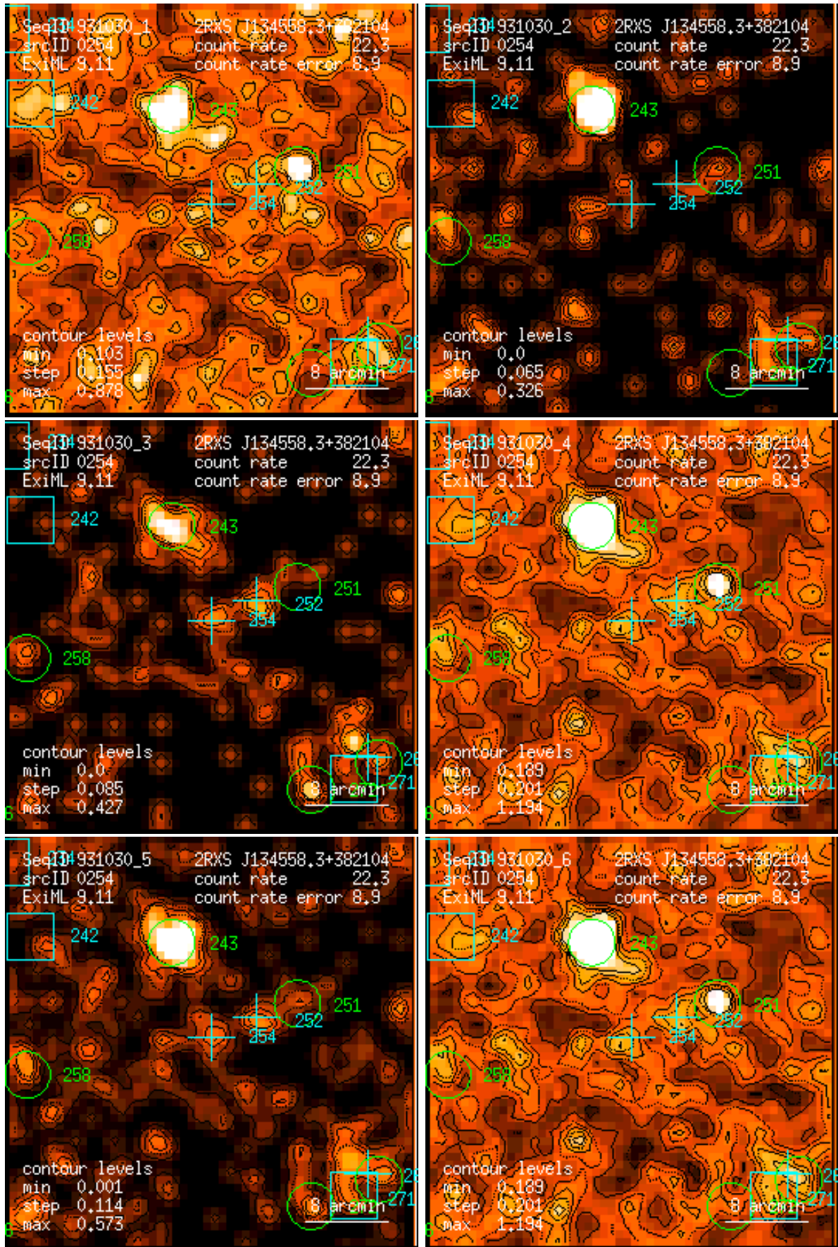
Figure 254: RASS 931030: detection 0254: band rate images, Gaussian filter: (1) PSPC channels 11 – 41, (2) 52 – 90, (3) 91 – 201, (4) 11 – 235, (5) 52 – 201, (6) 11 – 201. Broad band rates in counts/ks. Band rate contour levels in counts/ks/arcmin 2 .
