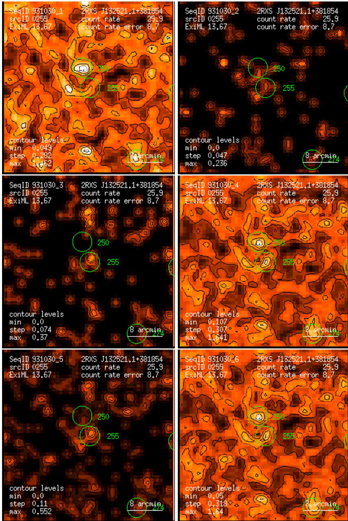
Figure 255: RASS 931030: detection 0255: band rate images, Gaussian filter: (1) PSPC channels 11 – 41, (2) 52 – 90, (3) 91 – 201, (4) 11 – 235, (5) 52 – 201, (6) 11 – 201. Broad band rates in counts/ks. Band rate contour levels in counts/ks/arcmin 2 .
