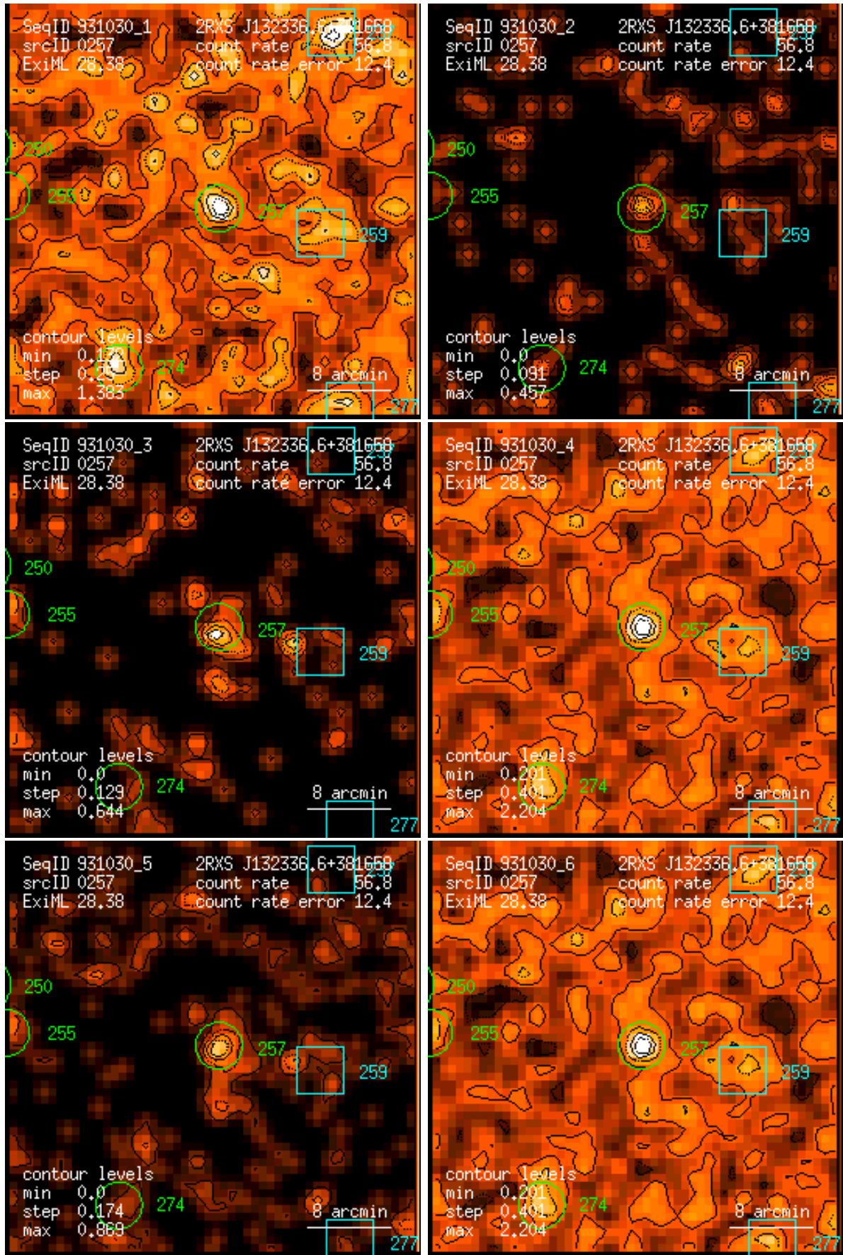
Figure 257: RASS 931030: detection 0257: band rate images, Gaussian filter: (1) PSPC channels 11 – 41, (2) 52 – 90, (3) 91 – 201, (4) 11 – 235, (5) 52 – 201, (6) 11 – 201. Broad band rates in counts/ks. Band rate contour levels in counts/ks/arcmin 2 .
