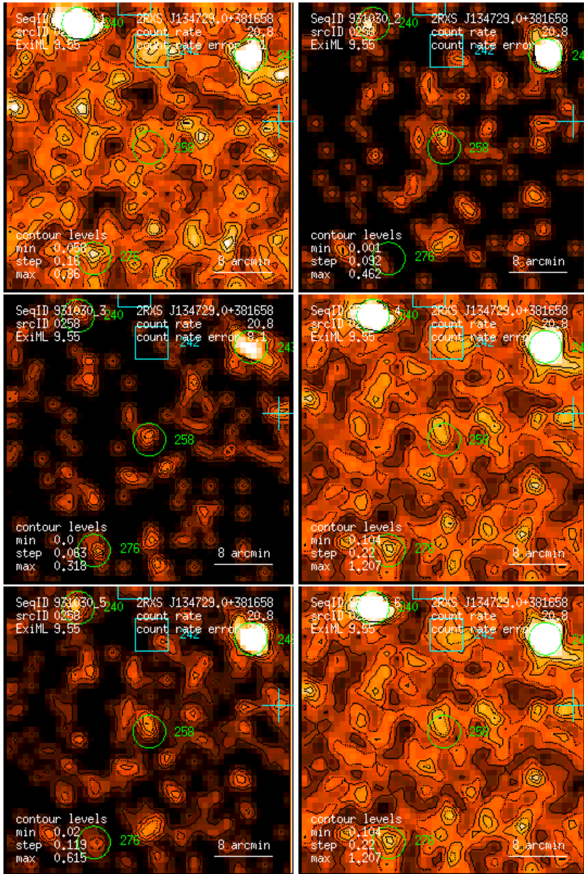
Figure 258: RASS 931030: detection 0258: band rate images, Gaussian filter: (1) PSPC channels 11 – 41, (2) 52 – 90, (3) 91 – 201, (4) 11 – 235, (5) 52 – 201, (6) 11 – 201. Broad band rates in counts/ks. Band rate contour levels in counts/ks/arcmin 2 .
