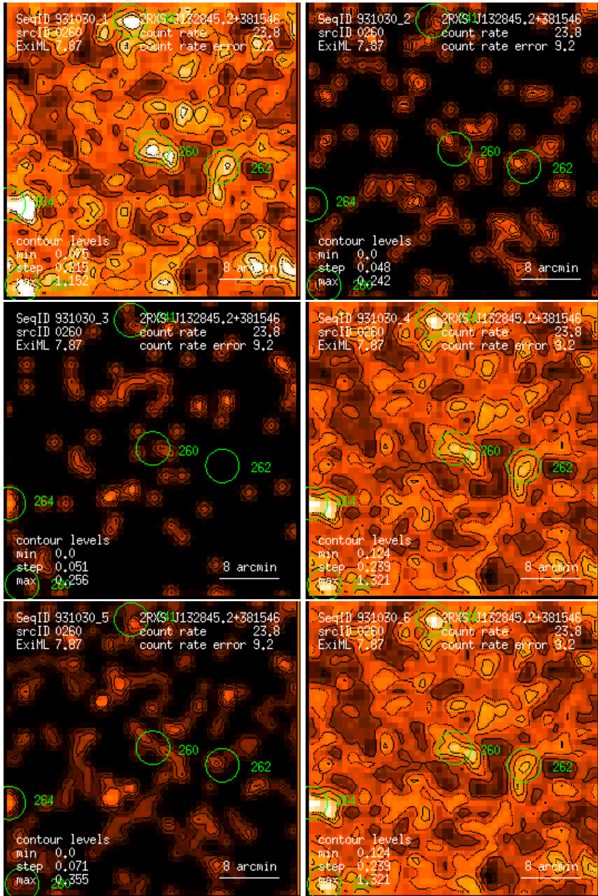
Figure 260: RASS 931030: detection 0260: band rate images, Gaussian filter: (1) PSPC channels 11 – 41, (2) 52 – 90, (3) 91 – 201, (4) 11 – 235, (5) 52 – 201, (6) 11 – 201. Broad band rates in counts/ks. Band rate contour levels in counts/ks/arcmin 2 .
