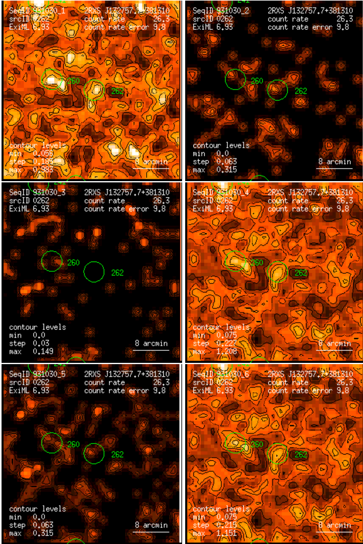
Figure 262: RASS 931030: detection 0262: band rate images, Gaussian filter: (1) PSPC channels 11 – 41, (2) 52 – 90, (3) 91 – 201, (4) 11 – 235, (5) 52 – 201, (6) 11 – 201. Broad band rates in counts/ks. Band rate contour levels in counts/ks/arcmin 2 .
