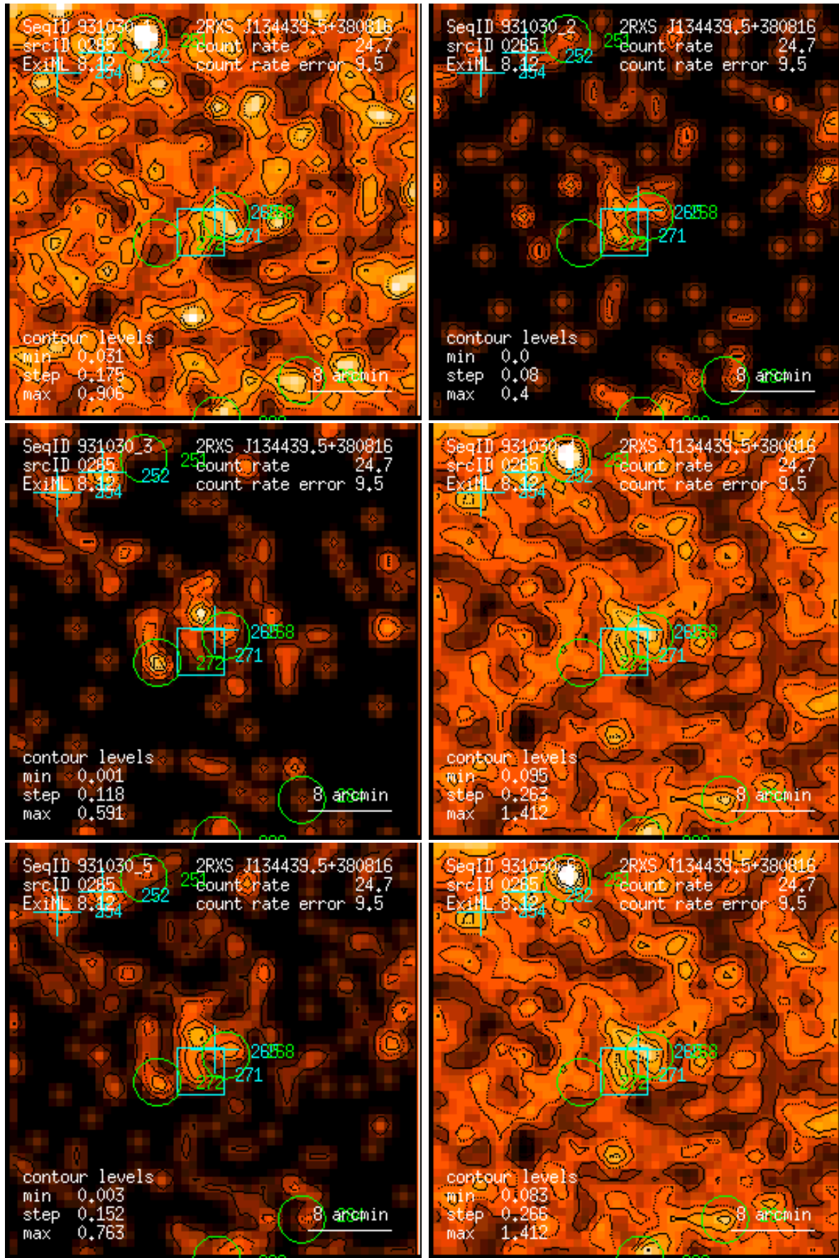
Figure 265: RASS 931030: detection 0265: band rate images, Gaussian filter: (1) PSPC channels 11 – 41, (2) 52 – 90, (3) 91 – 201, (4) 11 – 235, (5) 52 – 201, (6) 11 – 201. Broad band rates in counts/ks. Band rate contour levels in counts/ks/arcmin 2 .
