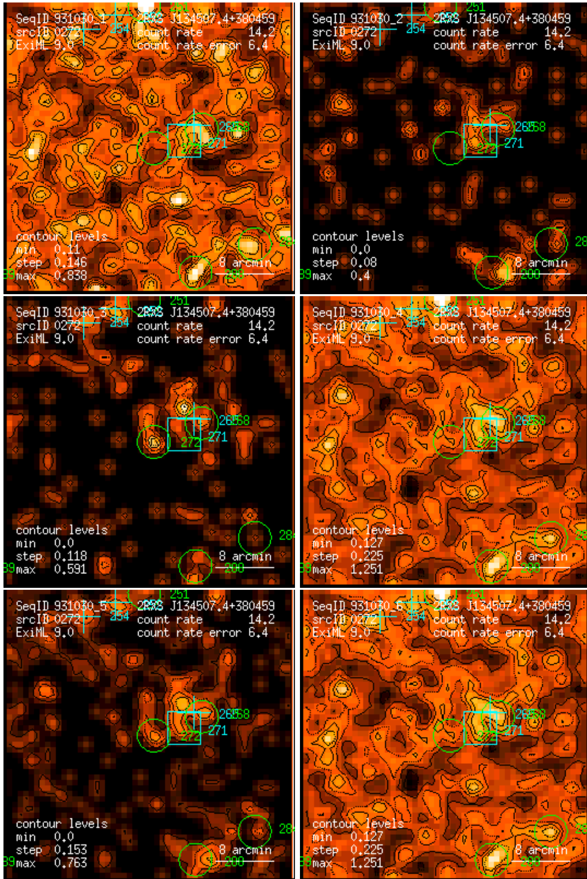
Figure 272: RASS 931030: detection 0272: band rate images, Gaussian filter: (1) PSPC channels 11 – 41, (2) 52 – 90, (3) 91 – 201, (4) 11 – 235, (5) 52 – 201, (6) 11 – 201. Broad band rates in counts/ks. Band rate contour levels in counts/ks/arcmin 2 .
