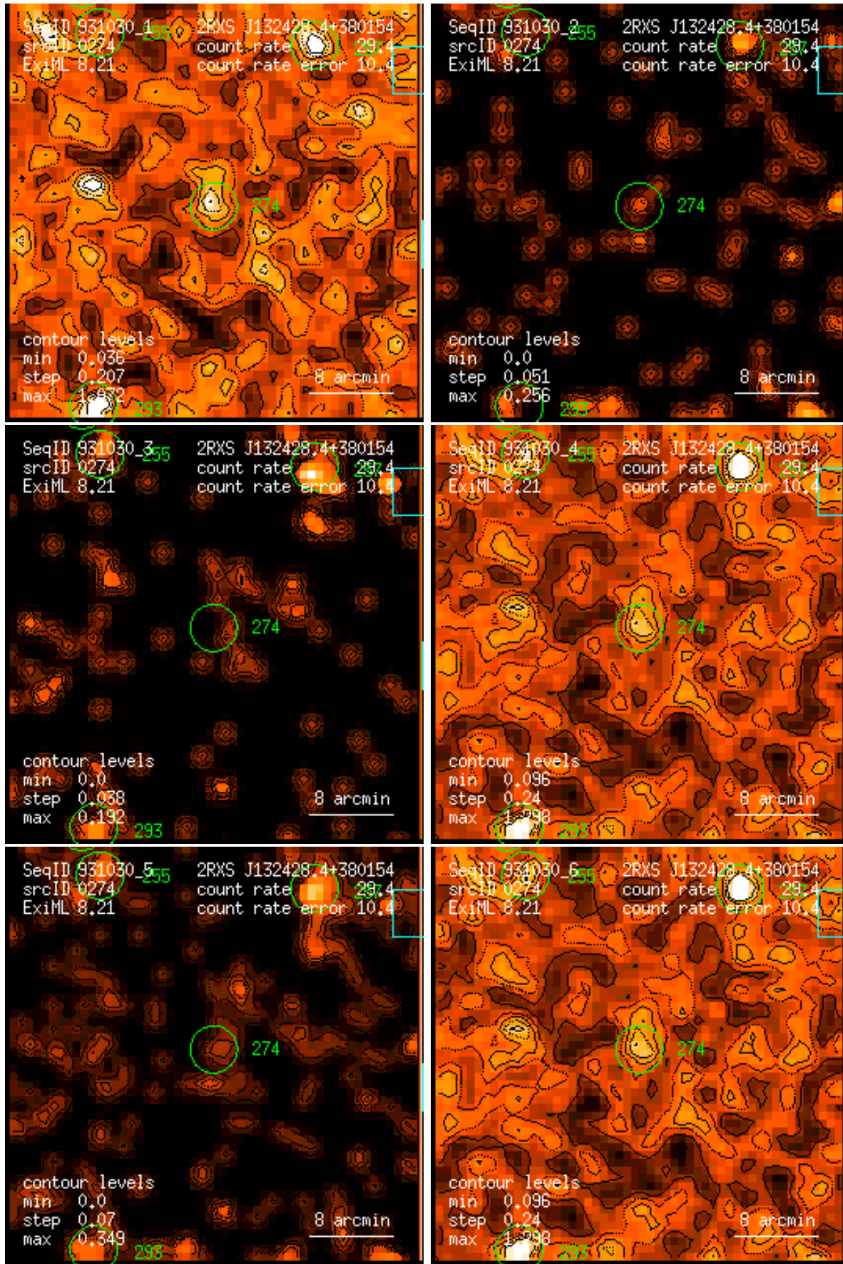
Figure 274: RASS 931030: detection 0274: band rate images, Gaussian filter: (1) PSPC channels 11 – 41, (2) 52 – 90, (3) 91 – 201, (4) 11 – 235, (5) 52 – 201, (6) 11 – 201. Broad band rates in counts/ks. Band rate contour levels in counts/ks/arcmin 2 .
