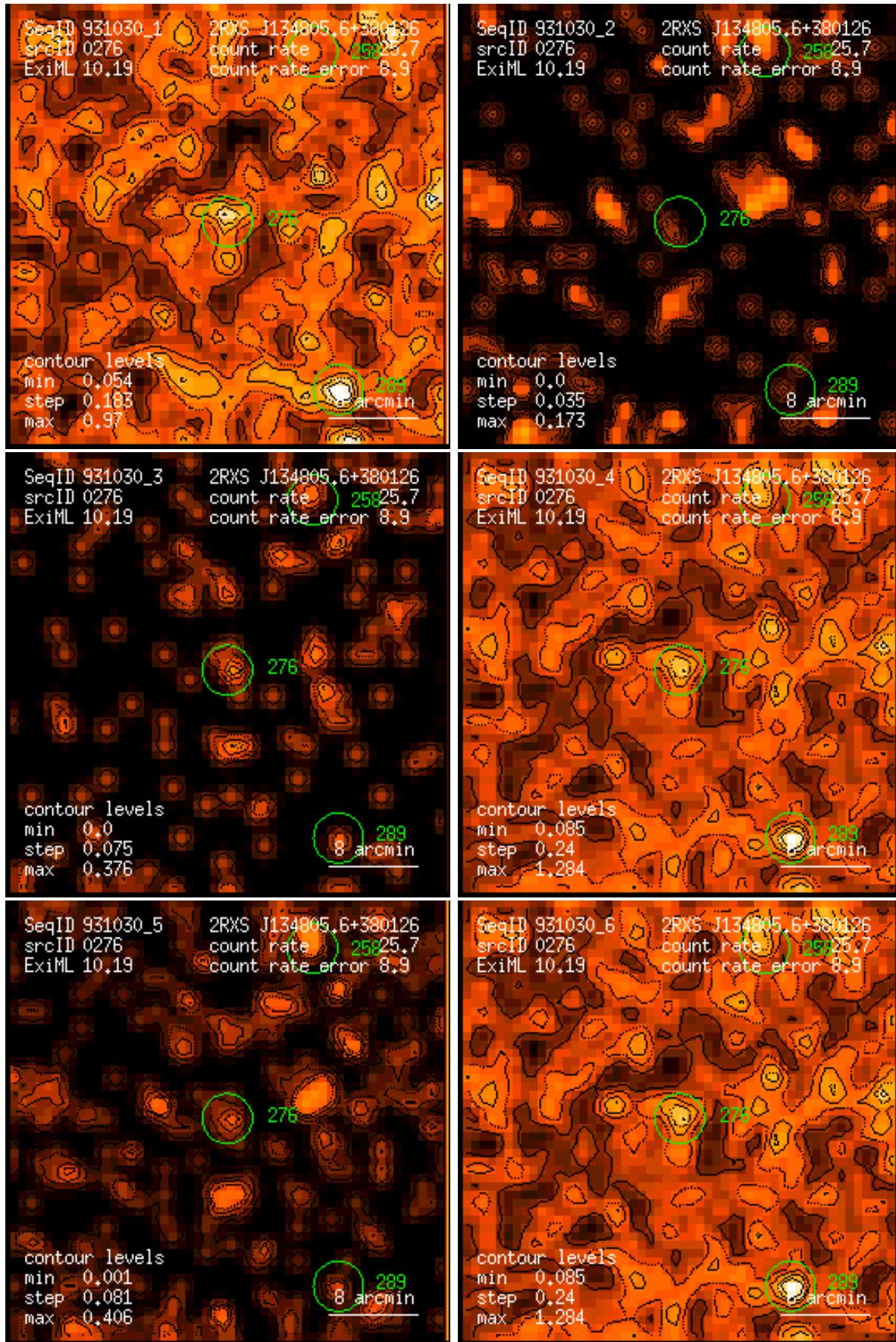
Figure 276: RASS 931030: detection 0276: band rate images, Gaussian filter: (1) PSPC channels 11 – 41, (2) 52 – 90, (3) 91 – 201, (4) 11 – 235, (5) 52 – 201, (6) 11 – 201. Broad band rates in counts/ks. Band rate contour levels in counts/ks/arcmin 2 .
