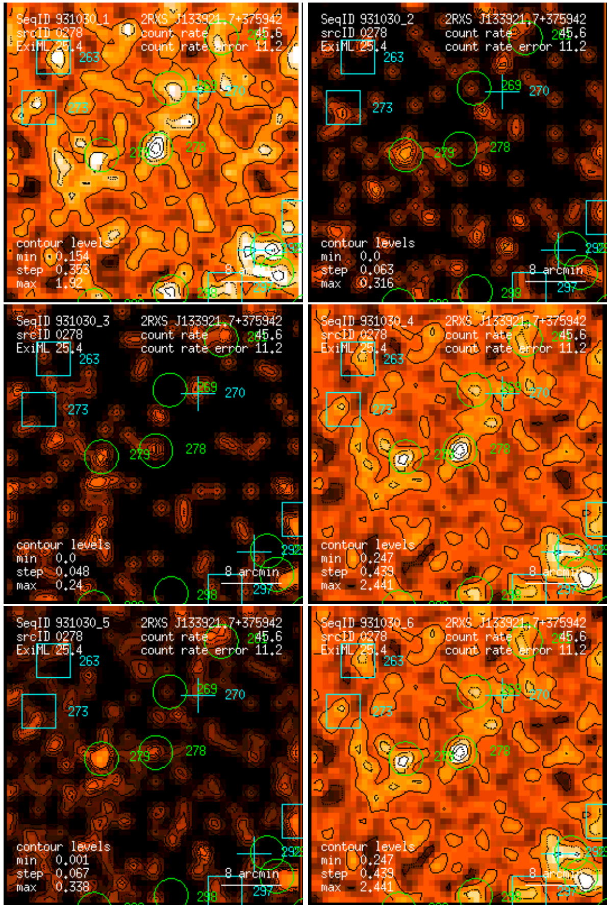
Figure 278: RASS 931030: detection 0278: band rate images, Gaussian filter: (1) PSPC channels 11 – 41, (2) 52 – 90, (3) 91 – 201, (4) 11 – 235, (5) 52 – 201, (6) 11 – 201. Broad band rates in counts/ks. Band rate contour levels in counts/ks/arcmin 2 .
