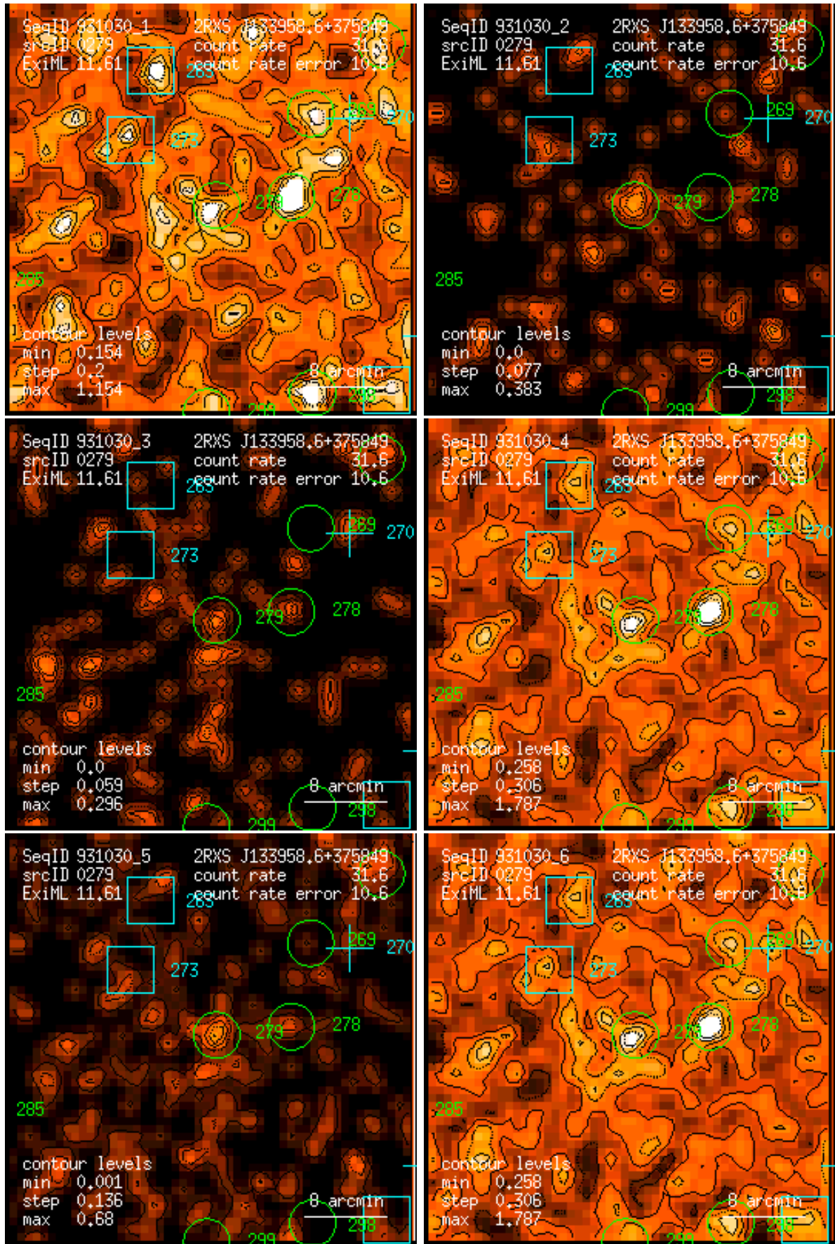
Figure 279: RASS 931030: detection 0279: band rate images, Gaussian filter: (1) PSPC channels 11 – 41, (2) 52 – 90, (3) 91 – 201, (4) 11 – 235, (5) 52 – 201, (6) 11 – 201. Broad band rates in counts/ks. Band rate contour levels in counts/ks/arcmin 2 .
