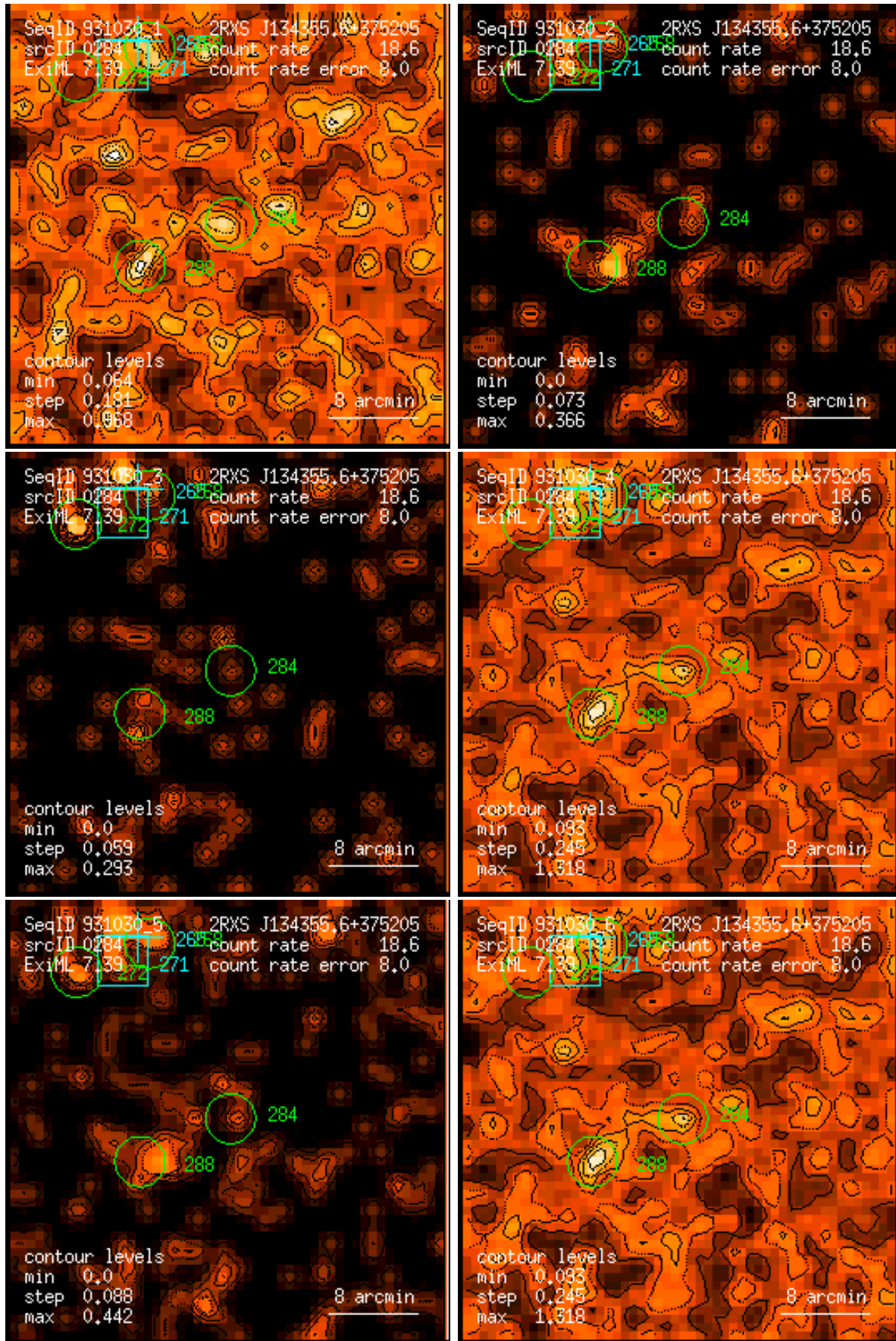
Figure 284: RASS 931030: detection 0284: band rate images, Gaussian filter: (1) PSPC channels 11 – 41, (2) 52 – 90, (3) 91 – 201, (4) 11 – 235, (5) 52 – 201, (6) 11 – 201. Broad band rates in counts/ks. Band rate contour levels in counts/ks/arcmin 2 .
