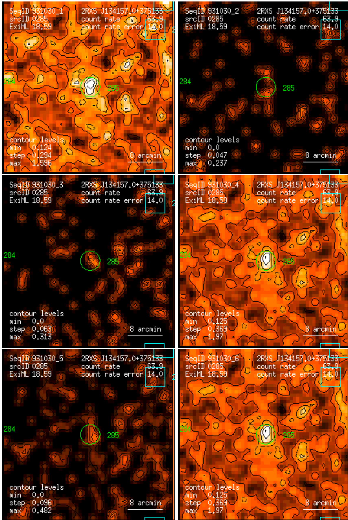
Figure 285: RASS 931030: detection 0285: band rate images, Gaussian filter: (1) PSPC channels 11 – 41, (2) 52 – 90, (3) 91 – 201, (4) 11 – 235, (5) 52 – 201, (6) 11 – 201. Broad band rates in counts/ks. Band rate contour levels in counts/ks/arcmin 2 .
