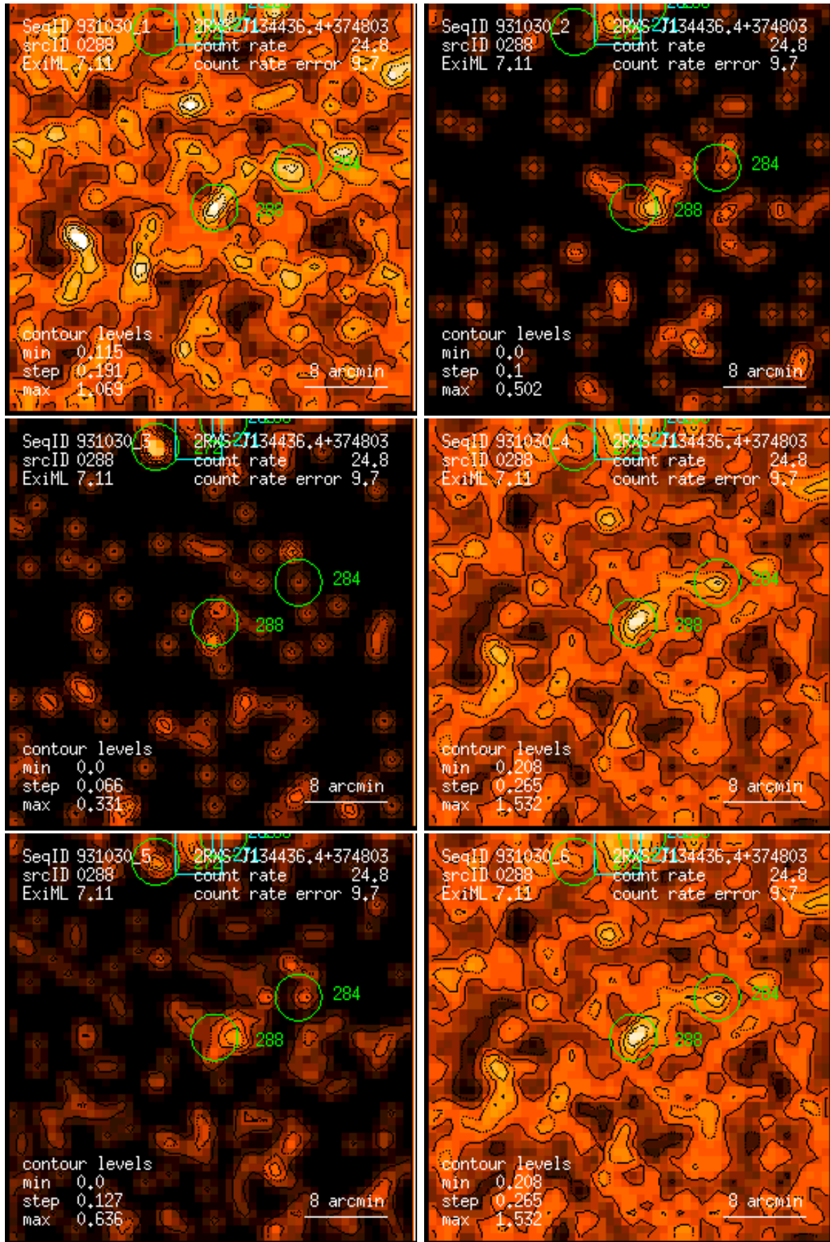
Figure 288: RASS 931030: detection 0288: band rate images, Gaussian filter: (1) PSPC channels 11 – 41, (2) 52 – 90, (3) 91 – 201, (4) 11 – 235, (5) 52 – 201, (6) 11 – 201. Broad band rates in counts/ks. Band rate contour levels in counts/ks/arcmin 2 .
