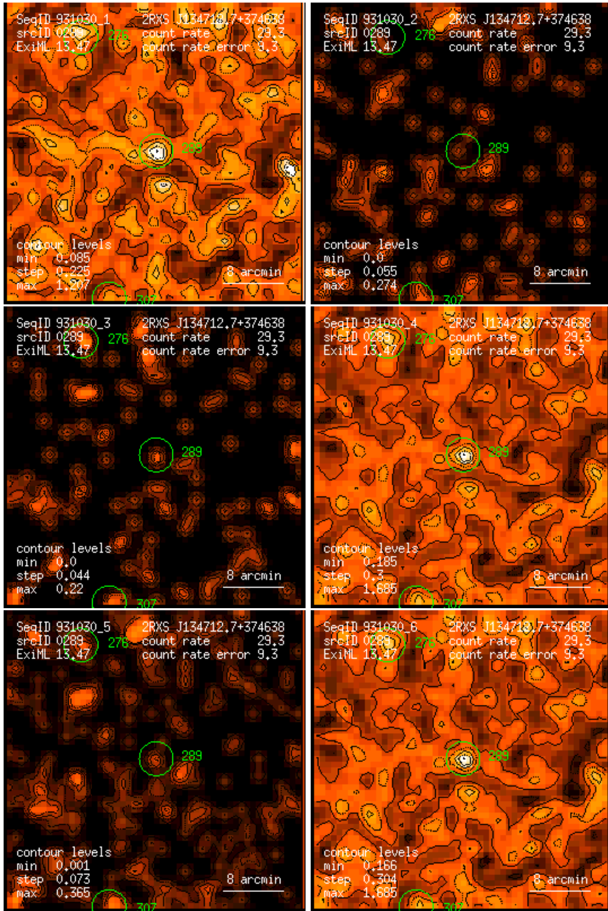
Figure 289: RASS 931030: detection 0289: band rate images, Gaussian filter: (1) PSPC channels 11 – 41, (2) 52 – 90, (3) 91 – 201, (4) 11 – 235, (5) 52 – 201, (6) 11 – 201. Broad band rates in counts/ks. Band rate contour levels in counts/ks/arcmin 2 .
