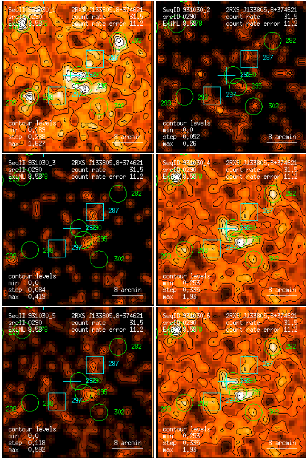
Figure 290: RASS 931030: detection 0290: band rate images, Gaussian filter: (1) PSPC channels 11 – 41, (2) 52 – 90, (3) 91 – 201, (4) 11 – 235, (5) 52 – 201, (6) 11 – 201. Broad band rates in counts/ks. Band rate contour levels in counts/ks/arcmin 2 .
