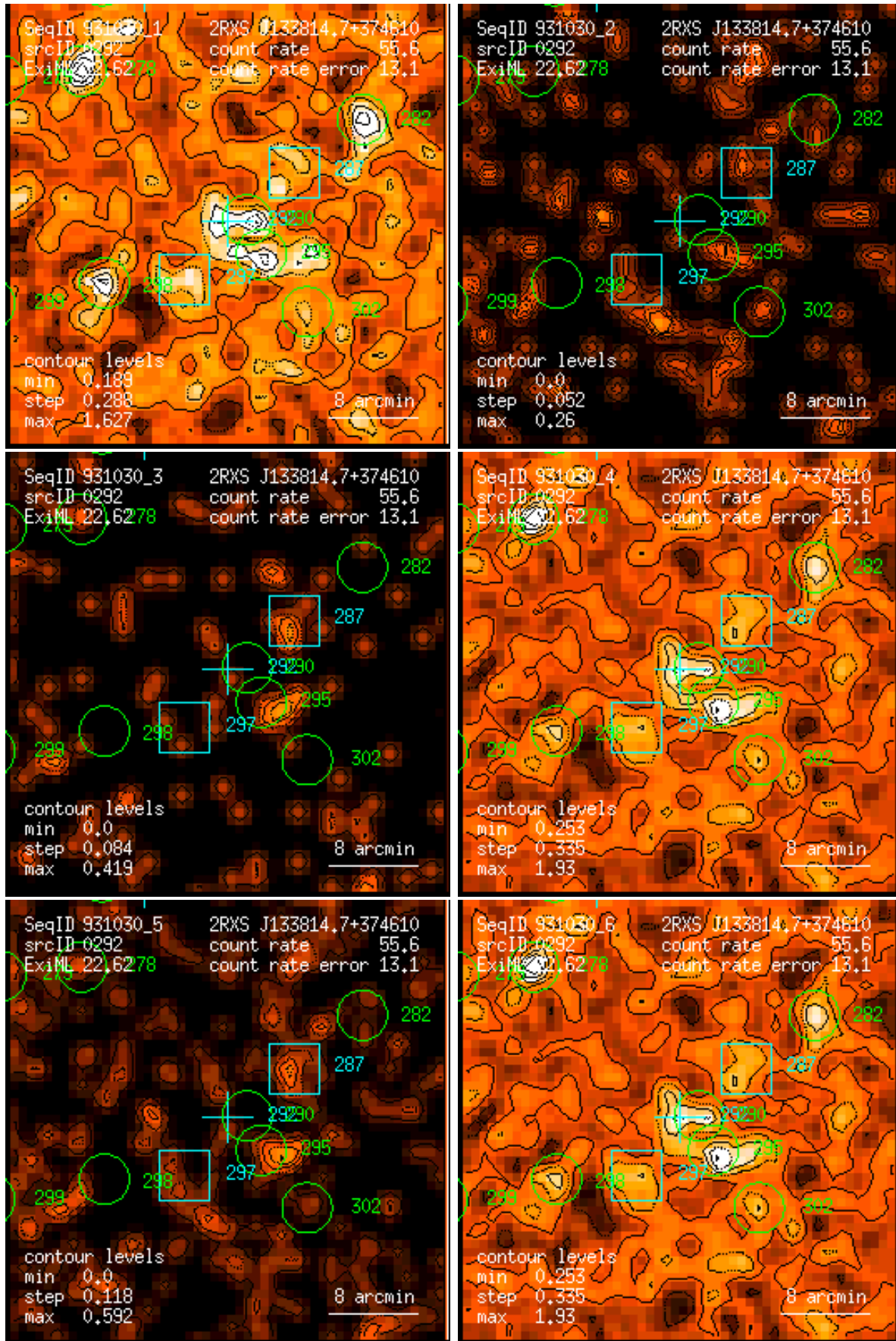
Figure 292: RASS 931030: detection 0292: band rate images, Gaussian filter: (1) PSPC channels 11 – 41, (2) 52 – 90, (3) 91 – 201, (4) 11 – 235, (5) 52 – 201, (6) 11 – 201. Broad band rates in counts/ks. Band rate contour levels in counts/ks/arcmin 2 .
