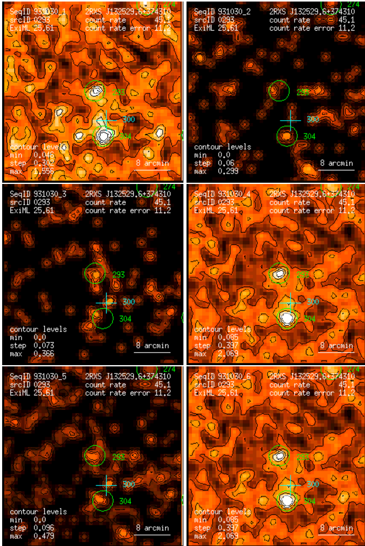
Figure 293: RASS 931030: detection 0293: band rate images, Gaussian filter: (1) PSPC channels 11 – 41, (2) 52 – 90, (3) 91 – 201, (4) 11 – 235, (5) 52 – 201, (6) 11 – 201. Broad band rates in counts/ks. Band rate contour levels in counts/ks/arcmin 2 .
