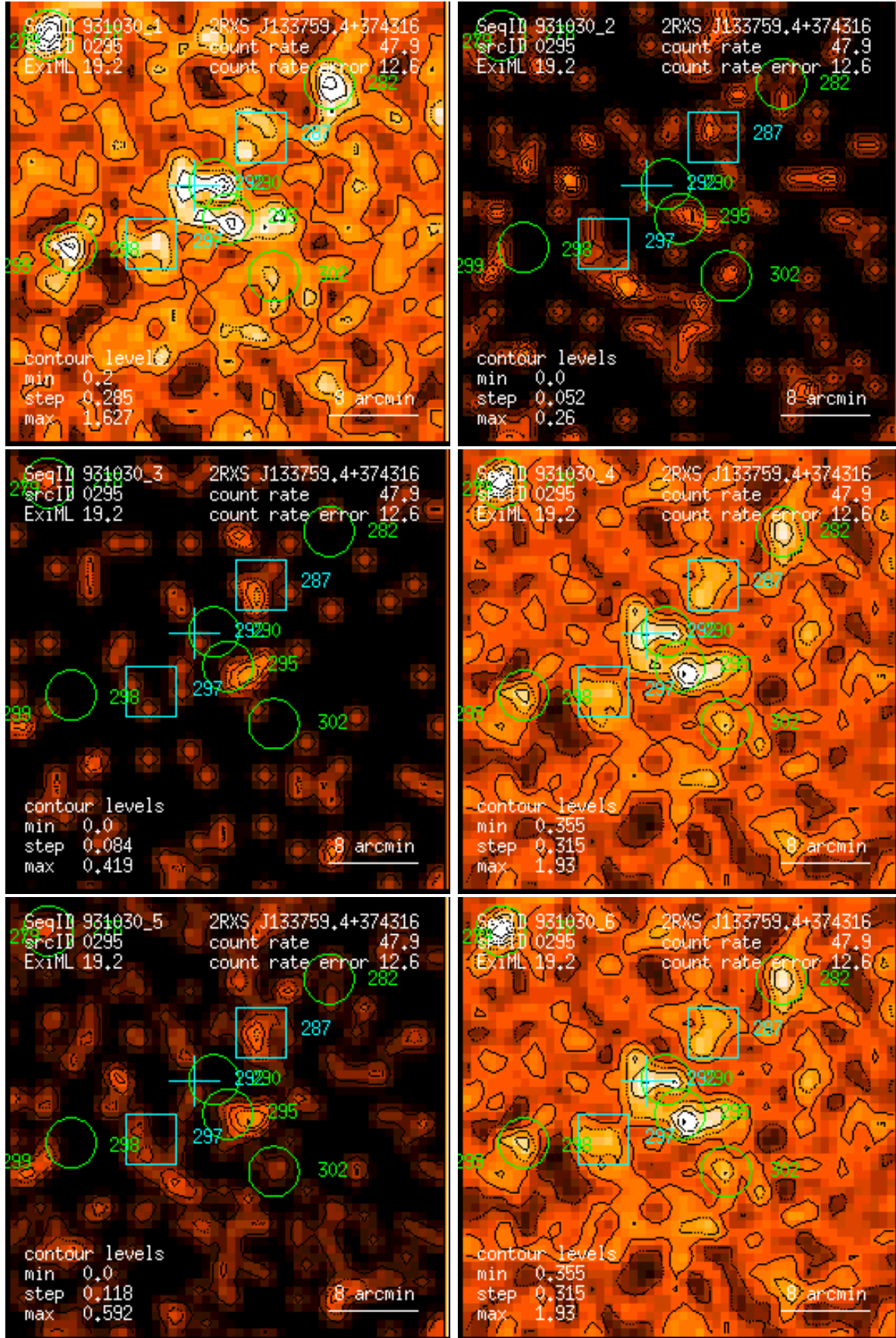
Figure 295: RASS 931030: detection 0295: band rate images, Gaussian filter: (1) PSPC channels 11 – 41, (2) 52 – 90, (3) 91 – 201, (4) 11 – 235, (5) 52 – 201, (6) 11 – 201. Broad band rates in counts/ks. Band rate contour levels in counts/ks/arcmin 2 .
