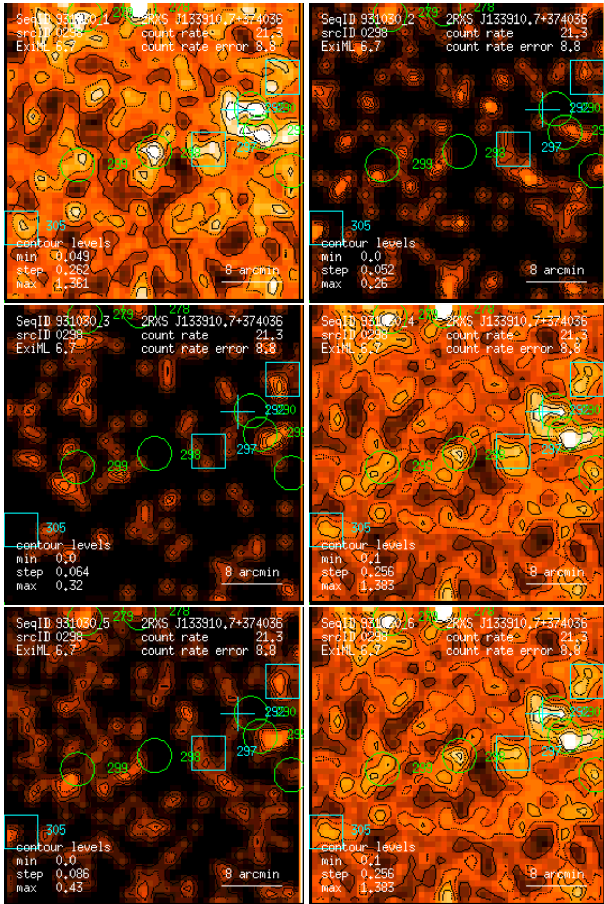
Figure 298: RASS 931030: detection 0298: band rate images, Gaussian filter: (1) PSPC channels 11 – 41, (2) 52 – 90, (3) 91 – 201, (4) 11 – 235, (5) 52 – 201, (6) 11 – 201. Broad band rates in counts/ks. Band rate contour levels in counts/ks/arcmin 2 .
