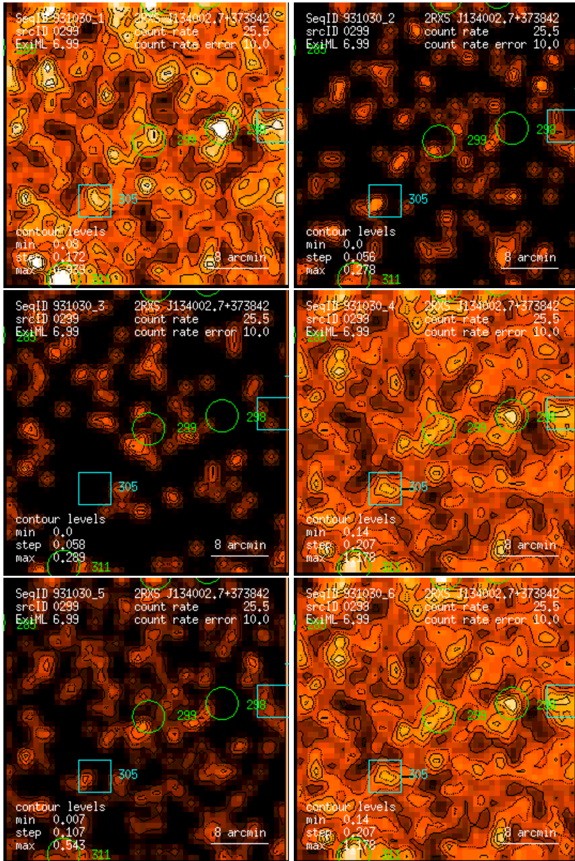
Figure 299: RASS 931030: detection 0299: band rate images, Gaussian filter: (1) PSPC channels 11 – 41, (2) 52 – 90, (3) 91 – 201, (4) 11 – 235, (5) 52 – 201, (6) 11 – 201. Broad band rates in counts/ks. Band rate contour levels in counts/ks/arcmin 2 .
