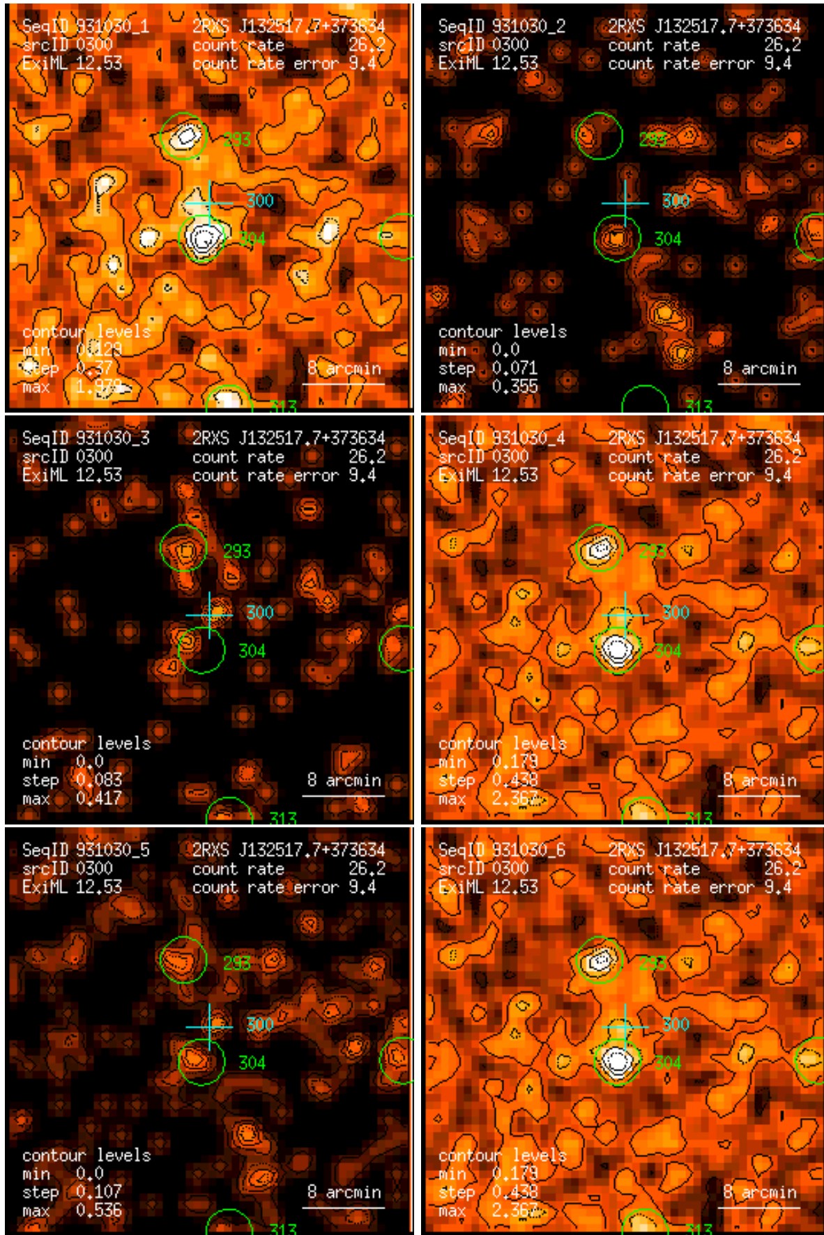
Figure 300: RASS 931030: detection 0300: band rate images, Gaussian filter: (1) PSPC channels 11 – 41, (2) 52 – 90, (3) 91 – 201, (4) 11 – 235, (5) 52 – 201, (6) 11 – 201. Broad band rates in counts/ks. Band rate contour levels in counts/ks/arcmin 2 .
