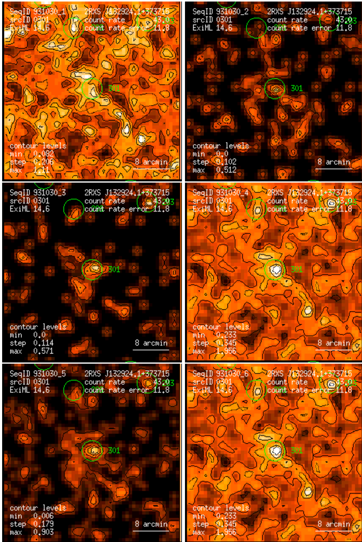
Figure 301: RASS 931030: detection 0301: band rate images, Gaussian filter: (1) PSPC channels 11 – 41, (2) 52 – 90, (3) 91 – 201, (4) 11 – 235, (5) 52 – 201, (6) 11 – 201. Broad band rates in counts/ks. Band rate contour levels in counts/ks/arcmin 2 .
