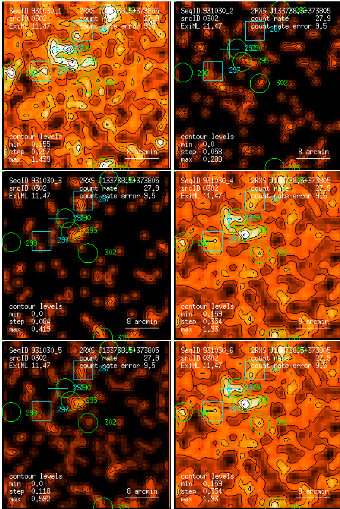
Figure 302: RASS 931030: detection 0302: band rate images, Gaussian filter: (1) PSPC channels 11 – 41, (2) 52 – 90, (3) 91 – 201, (4) 11 – 235, (5) 52 – 201, (6) 11 – 201. Broad band rates in counts/ks. Band rate contour levels in counts/ks/arcmin 2 .
