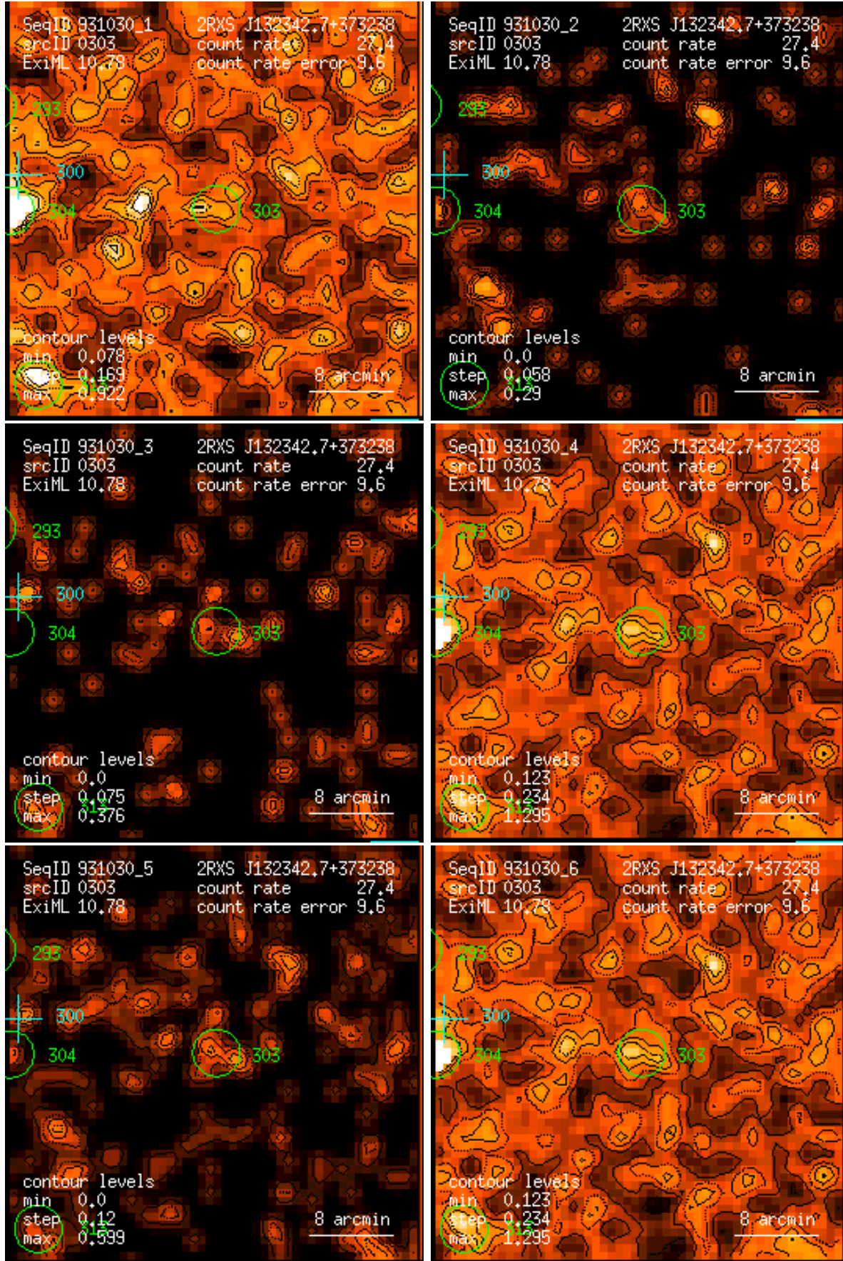
Figure 303: RASS 931030: detection 0303: band rate images, Gaussian filter: (1) PSPC channels 11 – 41, (2) 52 – 90, (3) 91 – 201, (4) 11 – 235, (5) 52 – 201, (6) 11 – 201. Broad band rates in counts/ks. Band rate contour levels in counts/ks/arcmin 2 .
