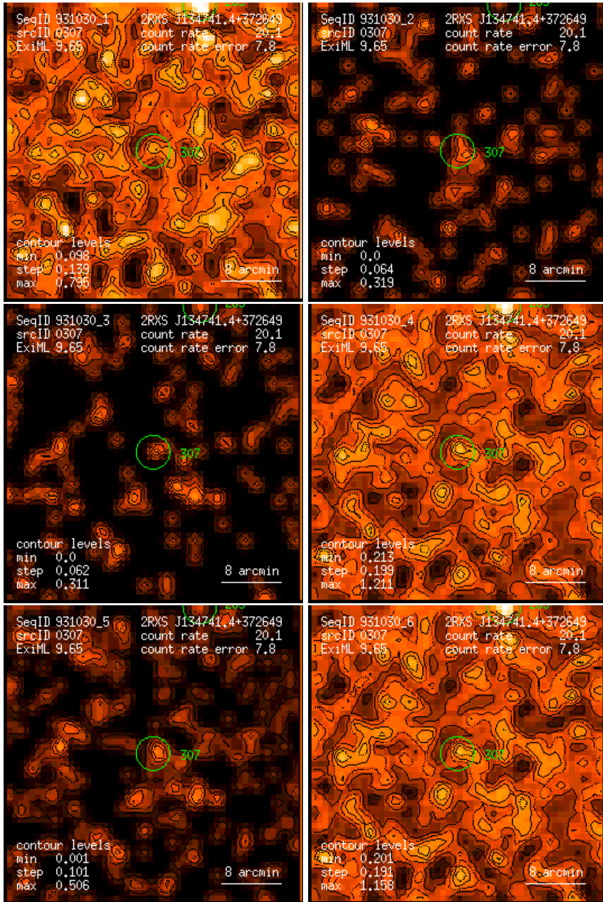
Figure 307: RASS 931030: detection 0307: band rate images, Gaussian filter: (1) PSPC channels 11 – 41, (2) 52 – 90, (3) 91 – 201, (4) 11 – 235, (5) 52 – 201, (6) 11 – 201. Broad band rates in counts/ks. Band rate contour levels in counts/ks/arcmin 2 .
