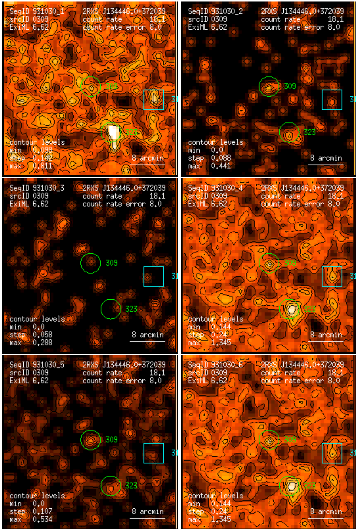
Figure 309: RASS 931030: detection 0309: band rate images, Gaussian filter: (1) PSPC channels 11 – 41, (2) 52 – 90, (3) 91 – 201, (4) 11 – 235, (5) 52 – 201, (6) 11 – 201. Broad band rates in counts/ks. Band rate contour levels in counts/ks/arcmin 2 .
