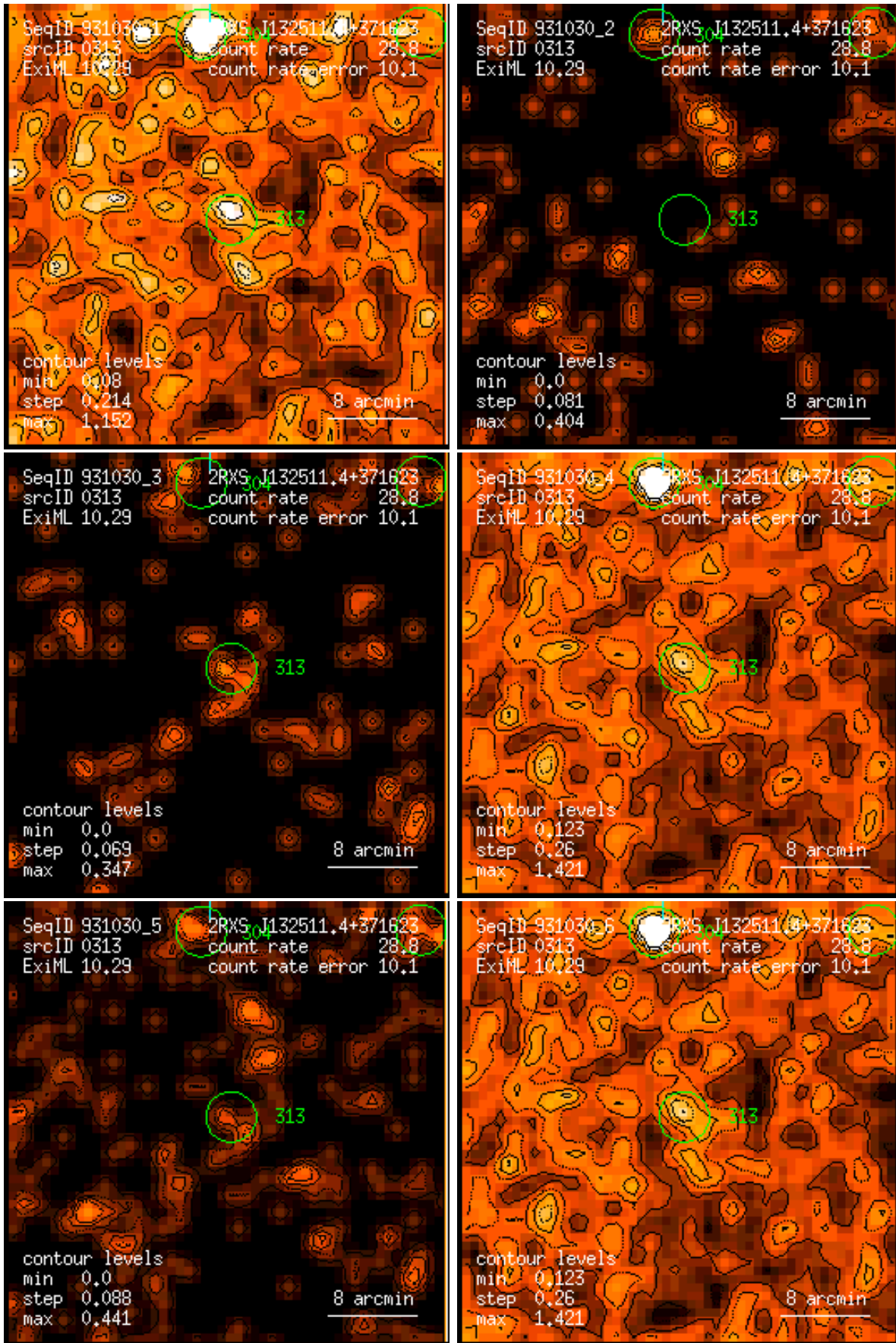
Figure 313: RASS 931030: detection 0313: band rate images, Gaussian filter: (1) PSPC channels 11 – 41, (2) 52 – 90, (3) 91 – 201, (4) 11 – 235, (5) 52 – 201, (6) 11 – 201. Broad band rates in counts/ks. Band rate contour levels in counts/ks/arcmin 2 .
