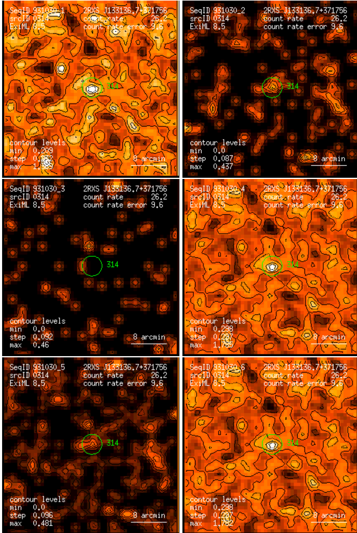
Figure 314: RASS 931030: detection 0314: band rate images, Gaussian filter: (1) PSPC channels 11 – 41, (2) 52 – 90, (3) 91 – 201, (4) 11 – 235, (5) 52 – 201, (6) 11 – 201. Broad band rates in counts/ks. Band rate contour levels in counts/ks/arcmin 2 .
