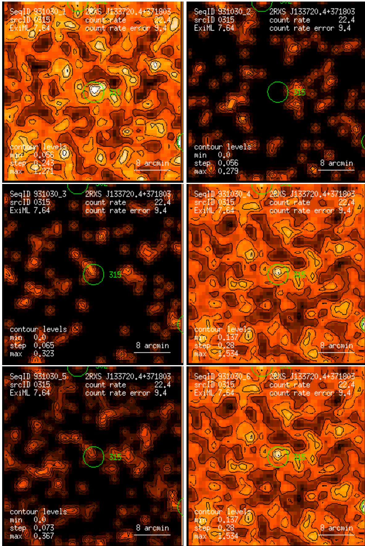
Figure 315: RASS 931030: detection 0315: band rate images, Gaussian filter: (1) PSPC channels 11 – 41, (2) 52 – 90, (3) 91 – 201, (4) 11 – 235, (5) 52 – 201, (6) 11 – 201. Broad band rates in counts/ks. Band rate contour levels in counts/ks/arcmin 2 .
