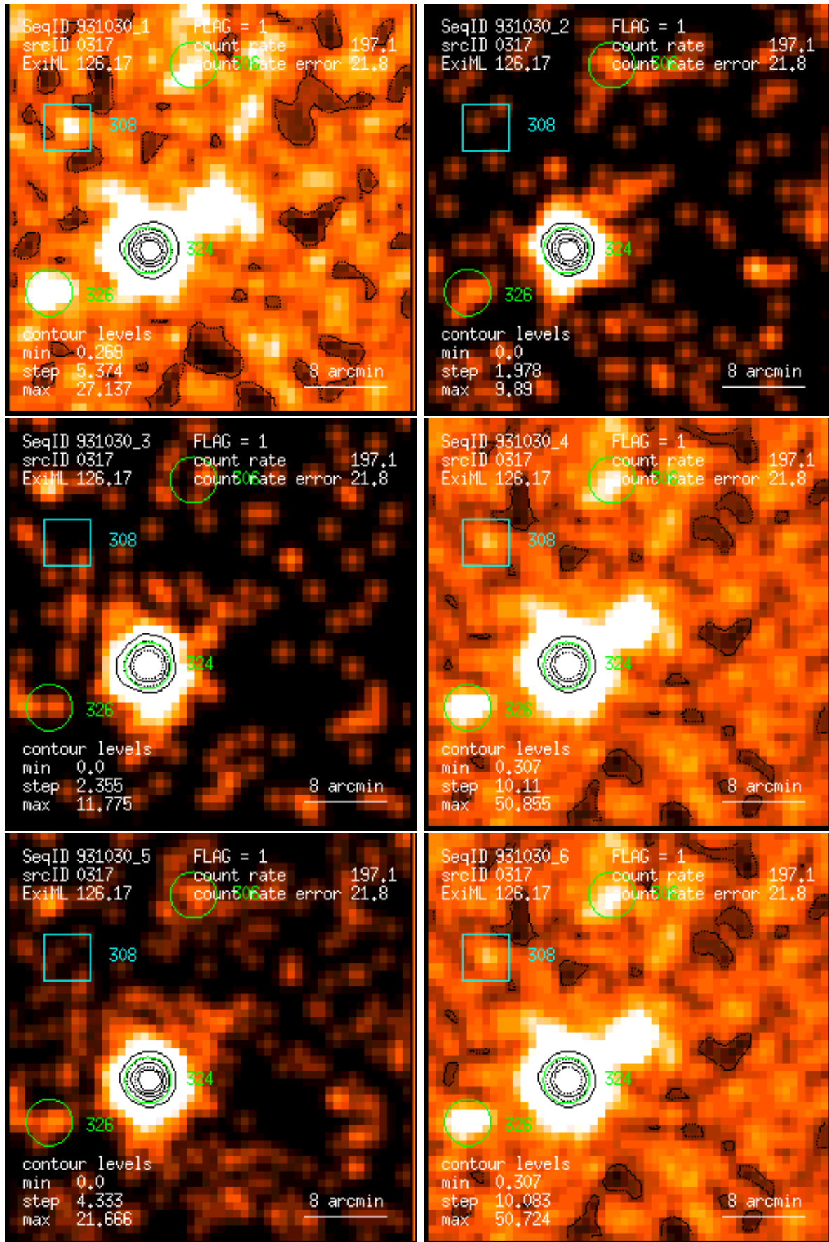
Figure 317: RASS 931030: detection 0317: band rate images, Gaussian filter: (1) PSPC channels 11 – 41, (2) 52 – 90, (3) 91 – 201, (4) 11 – 235, (5) 52 – 201, (6) 11 – 201. Broad band rates in counts/ks. Band rate contour levels in counts/ks/arcmin 2 .
