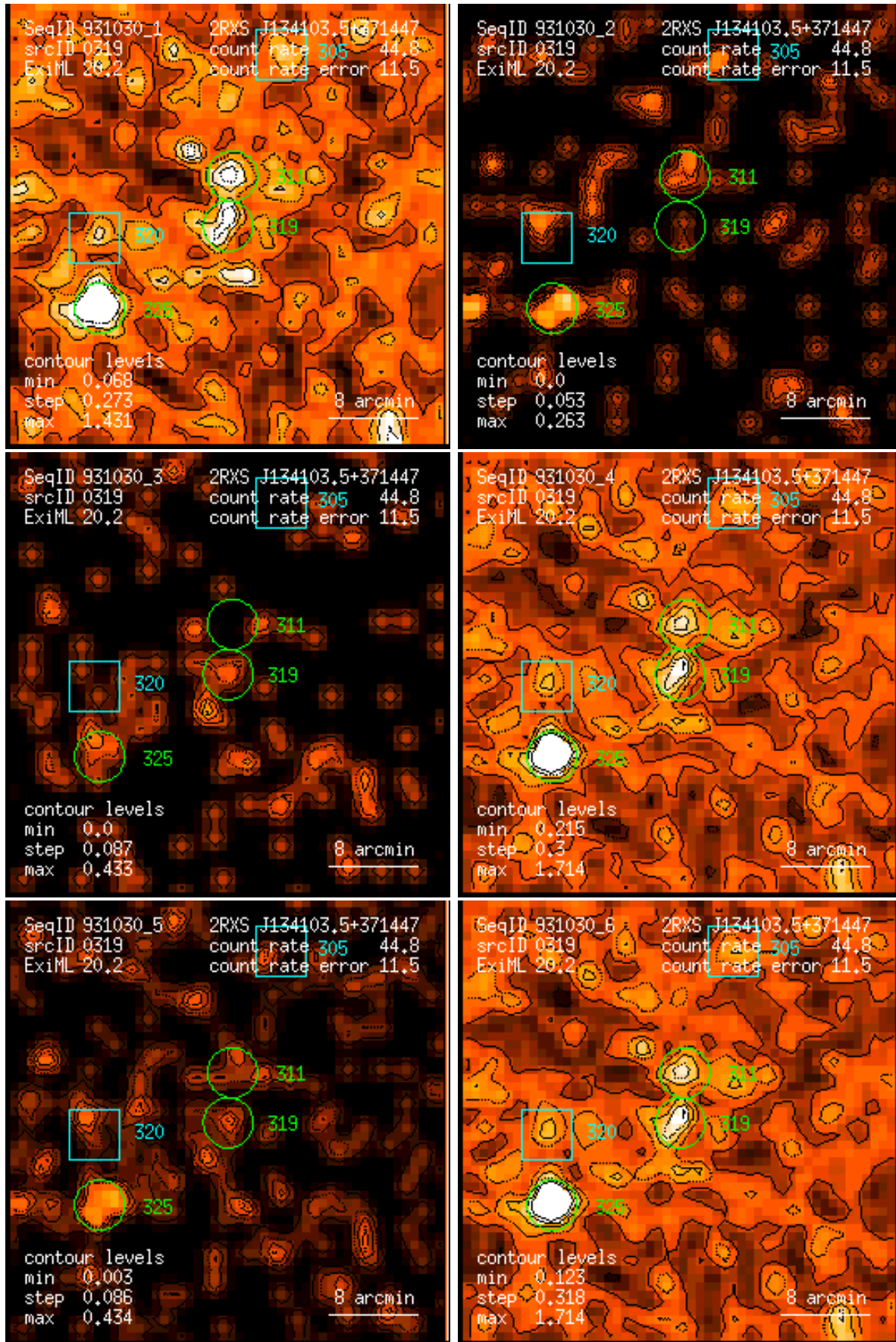
Figure 319: RASS 931030: detection 0319: band rate images, Gaussian filter: (1) PSPC channels 11 – 41, (2) 52 – 90, (3) 91 – 201, (4) 11 – 235, (5) 52 – 201, (6) 11 – 201. Broad band rates in counts/ks. Band rate contour levels in counts/ks/arcmin 2 .
