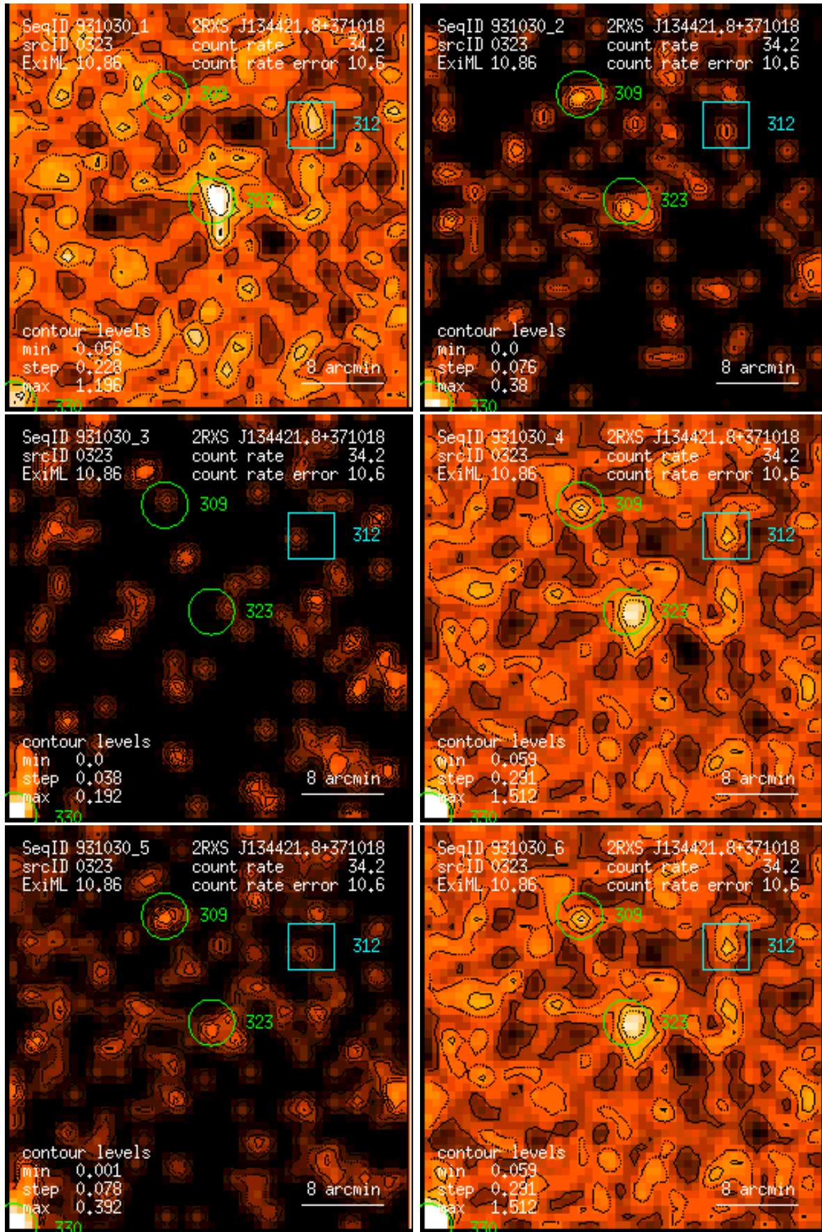
Figure 323: RASS 931030: detection 0323: band rate images, Gaussian filter: (1) PSPC channels 11 – 41, (2) 52 – 90, (3) 91 – 201, (4) 11 – 235, (5) 52 – 201, (6) 11 – 201. Broad band rates in counts/ks. Band rate contour levels in counts/ks/arcmin 2 .
