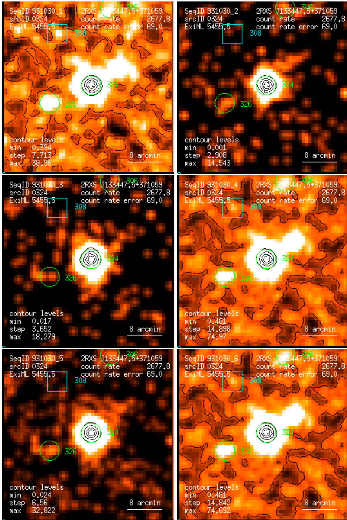
Figure 324: RASS 931030: detection 0324: band rate images, Gaussian filter: (1) PSPC channels 11 – 41, (2) 52 – 90, (3) 91 – 201, (4) 11 – 235, (5) 52 – 201, (6) 11 – 201. Broad band rates in counts/ks. Band rate contour levels in counts/ks/arcmin 2 .
