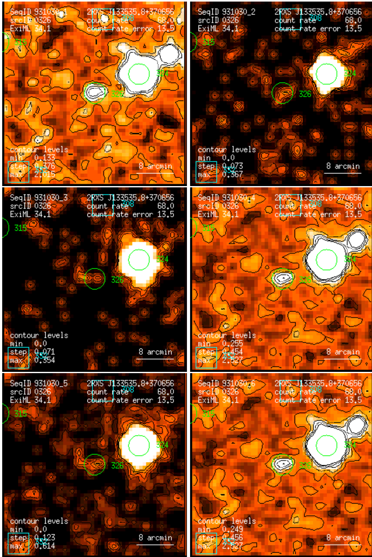
Figure 326: RASS 931030: detection 0326: band rate images, Gaussian filter: (1) PSPC channels 11 – 41, (2) 52 – 90, (3) 91 – 201, (4) 11 – 235, (5) 52 – 201, (6) 11 – 201. Broad band rates in counts/ks. Band rate contour levels in counts/ks/arcmin 2 .
