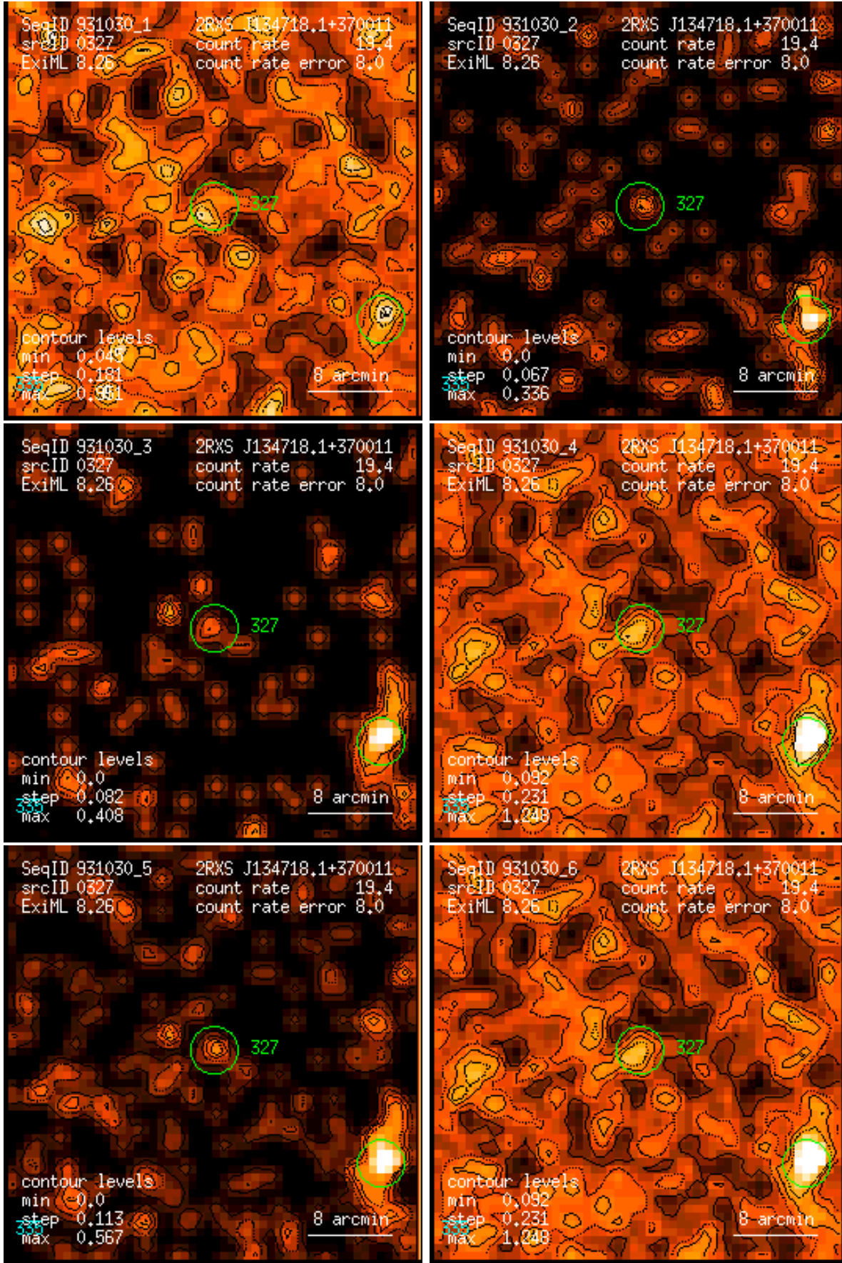
Figure 327: RASS 931030: detection 0327: band rate images, Gaussian filter: (1) PSPC channels 11 – 41, (2) 52 – 90, (3) 91 – 201, (4) 11 – 235, (5) 52 – 201, (6) 11 – 201. Broad band rates in counts/ks. Band rate contour levels in counts/ks/arcmin 2 .
