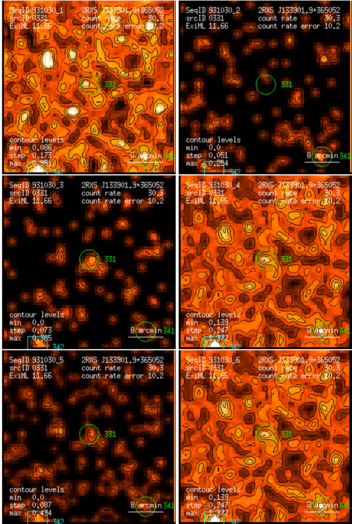
Figure 331: RASS 931030: detection 0331: band rate images, Gaussian filter: (1) PSPC channels 11 – 41, (2) 52 – 90, (3) 91 – 201, (4) 11 – 235, (5) 52 – 201, (6) 11 – 201. Broad band rates in counts/ks. Band rate contour levels in counts/ks/arcmin 2 .
