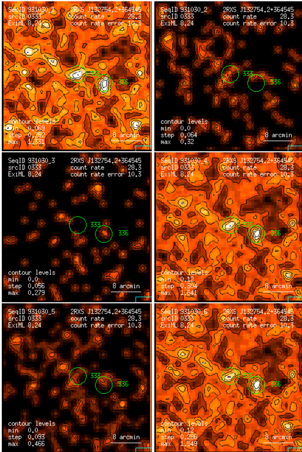
Figure 333: RASS 931030: detection 0333: band rate images, Gaussian filter: (1) PSPC channels 11 – 41, (2) 52 – 90, (3) 91 – 201, (4) 11 – 235, (5) 52 – 201, (6) 11 – 201. Broad band rates in counts/ks. Band rate contour levels in counts/ks/arcmin 2 .
