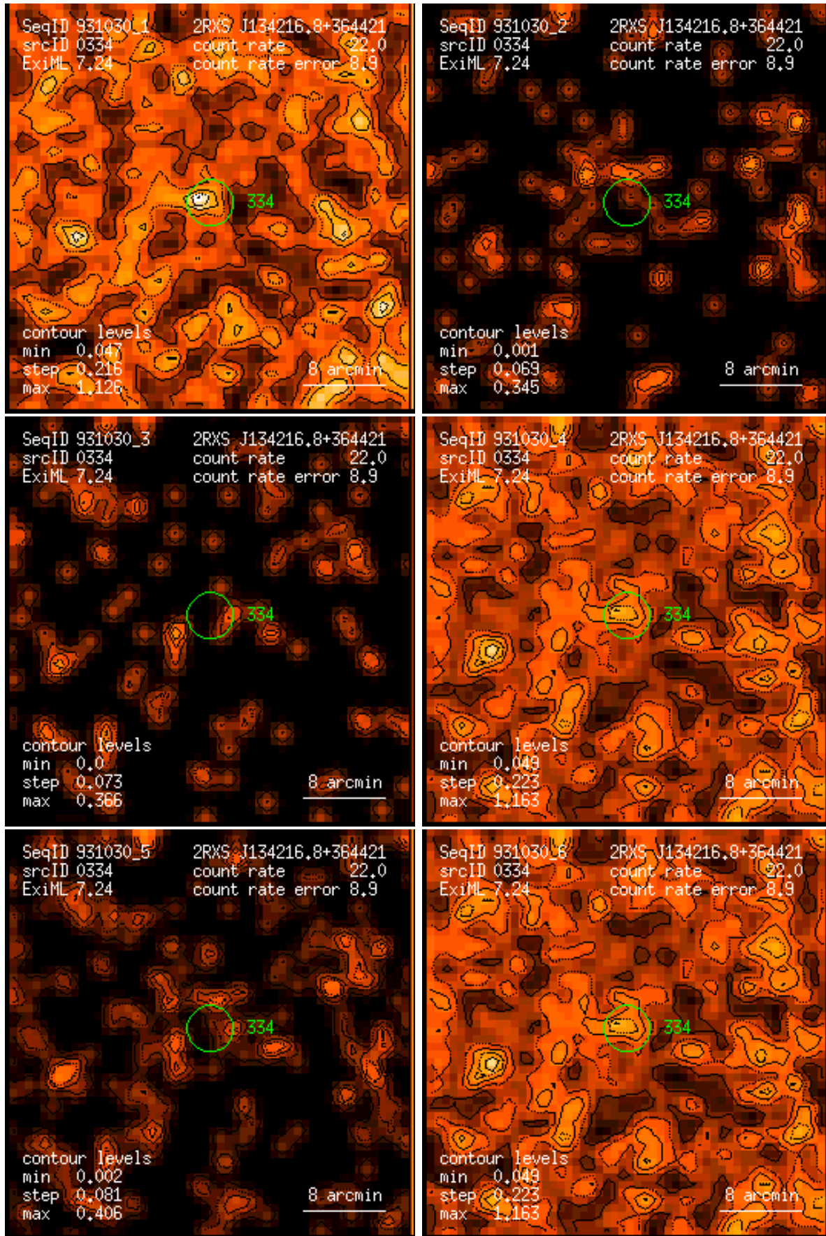
Figure 334: RASS 931030: detection 0334: band rate images, Gaussian filter: (1) PSPC channels 11 – 41, (2) 52 – 90, (3) 91 – 201, (4) 11 – 235, (5) 52 – 201, (6) 11 – 201. Broad band rates in counts/ks. Band rate contour levels in counts/ks/arcmin 2 .
