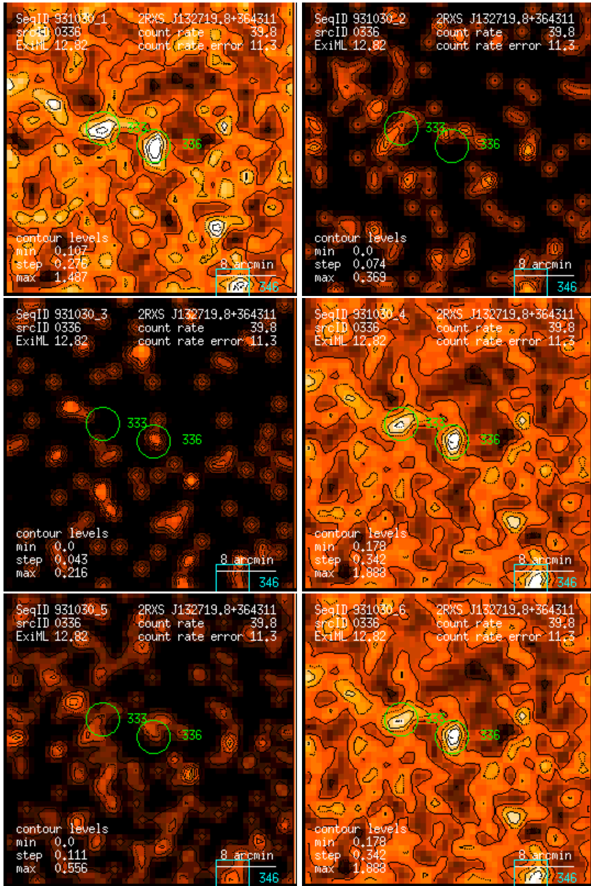
Figure 336: RASS 931030: detection 0336: band rate images, Gaussian filter: (1) PSPC channels 11 – 41, (2) 52 – 90, (3) 91 – 201, (4) 11 – 235, (5) 52 – 201, (6) 11 – 201. Broad band rates in counts/ks. Band rate contour levels in counts/ks/arcmin 2 .
